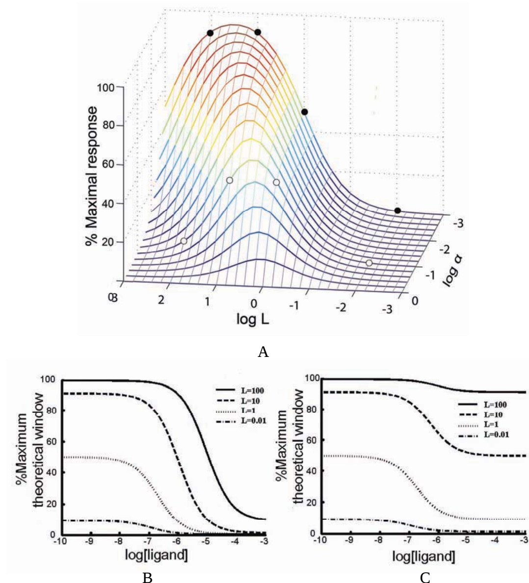
Figure. 8 A) Three-dimensional mesh of the percentage of maximum theoretical window for hypothetical inverse agonists with continuous intrinsic efficacy ( \alpha ) values between 0.001 to 1 on hypothetical receptors with continuous ratios of active versus inactive receptors ( L values) between 0.001 to 1000. In figure 8B, concentration-response curves are shown for receptors with L values of 0.01, 1, 10 and 100 for a strong inverse agonist with an \alpha value of 0.001 (closed circles in figure 8A). Similarly, in figure 8C, concentration-response curves are shown for a weak inverse agonist with an \alpha value of 0.1 (open circles in figure 8A).
