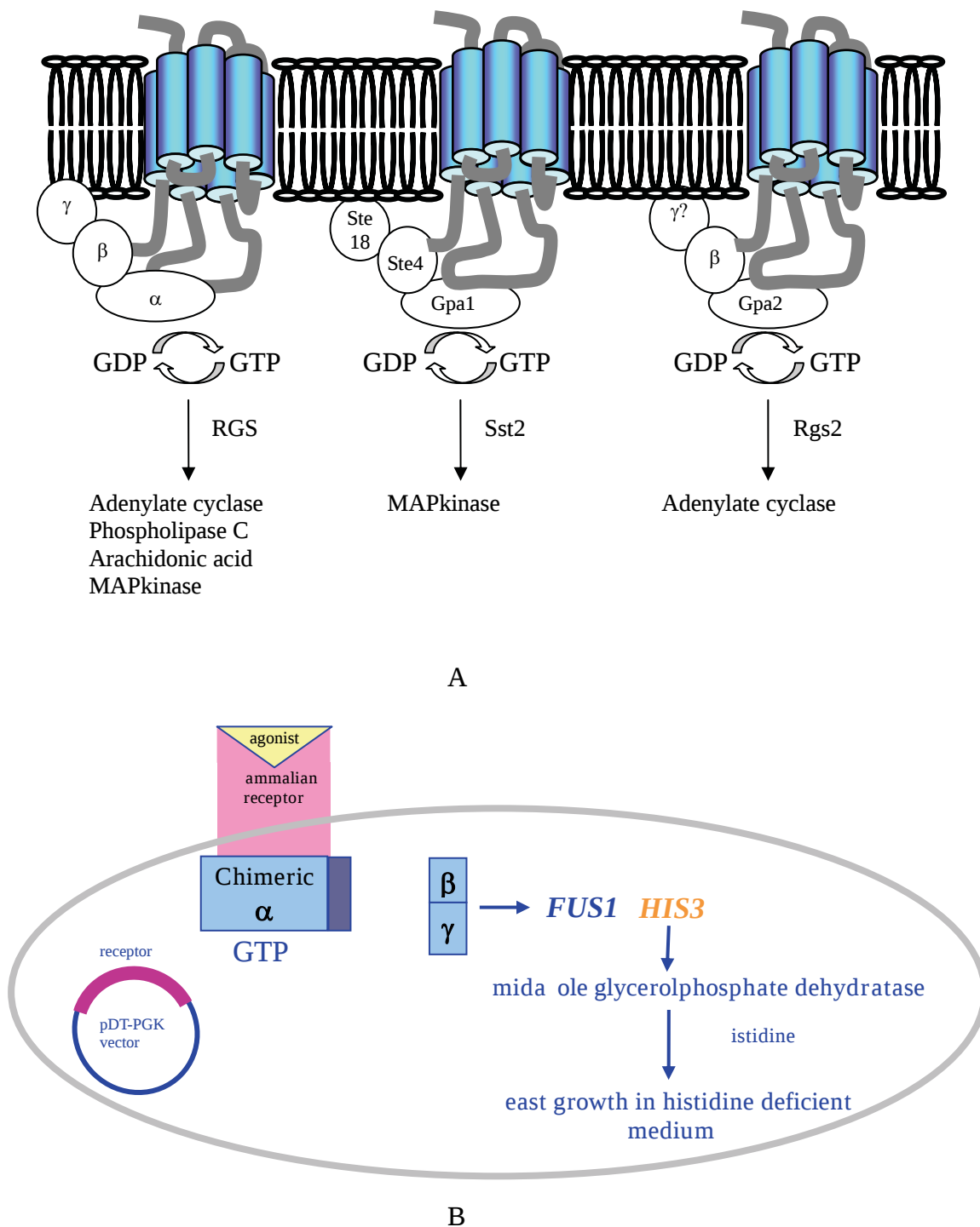
Figure 1. A) Schematic drawing of GPCR activation in yeast and mammalian cells. B) Schematic drawing of GPCR activation in genetically modified yeasts. When heterologously expressed mammalian receptors were activated by agonists, yeast \beta and \gamma subunits disassemble from the \alpha subunit and activate the Fus promoter which in turn activates the transcription of reporter genes, for example imidazole glycerolphosphatedehydratase. This enzyme enables yeast cells to synthesize histidine allowing them to grow in histidine-deficient medium. Gpa: G protein alpha, Gpr: G protein-coupled receptor, RGS/Rgs: regulators of G protein signaling, Sst2: supersensitivity to pheromone, Ste: sterility
