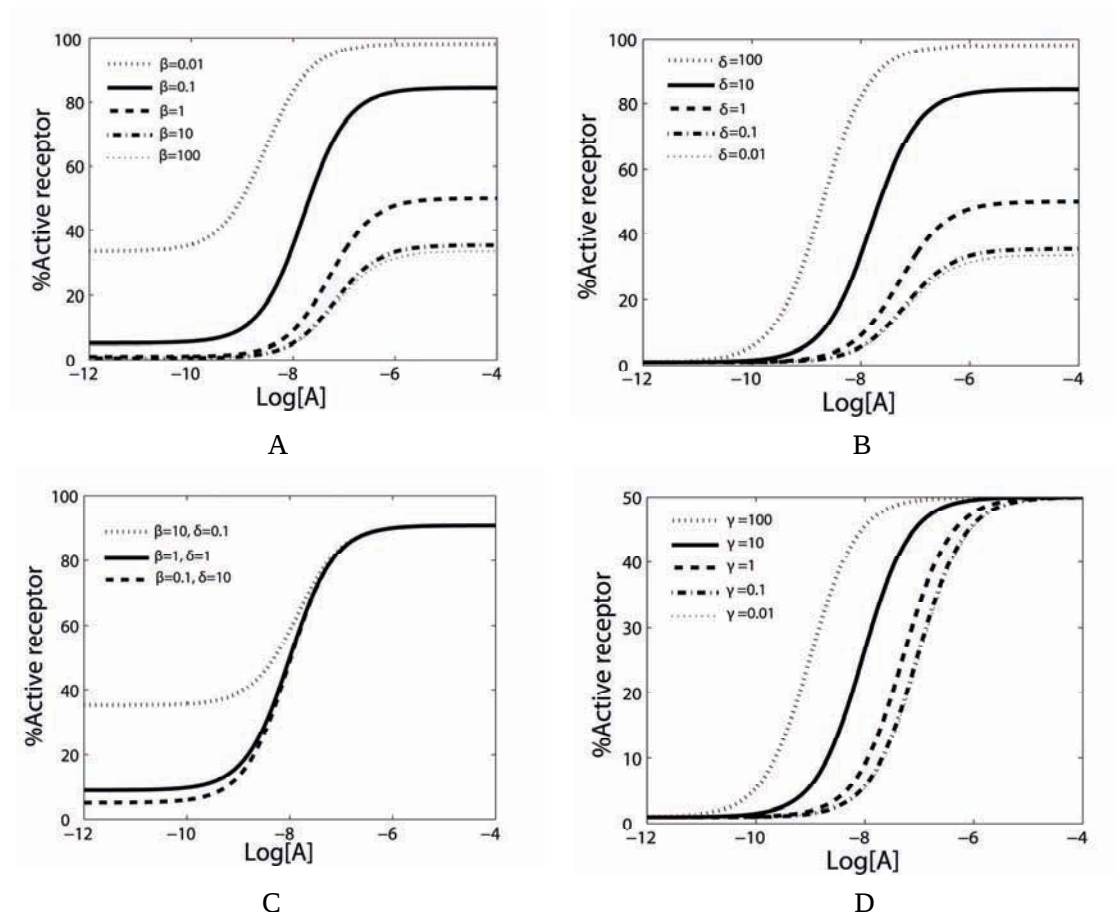
Figure 3. Simulation of the allosteric effect caused by variation of the parameters of an allosteric modulator. The following parameters are consistent throughout K = 100 nM, M = 100 nM, \alpha = 100 , and [C] = 100 nM). In addition the L value of the receptor is set at 0.1 in figures 3A, 3B, 3D and 1 in figure 3C.
