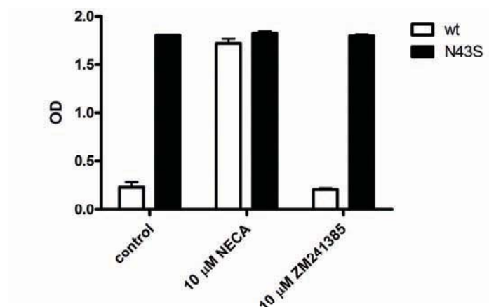
Figure. 3 Growth of yeast cells expressing the wild-type adenosine A_{2B} receptor or the N43S mutant receptor. Growth was measured in the absence (control) or presence of 10 \mu M NECA or 10 \mu M ZM241385. Each experiment was repeated 3 times, of which the means \pm SEM are shown. *** p < 0.001 , student's unpaired t test.
