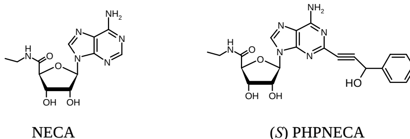
Figure 6. Chemical structure of two adenosine derived A 2B agonists: NECA and (S) PHPNECA.
