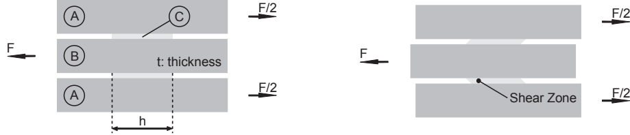
Figure 6.4: Miyauchi Test; Left: State before performing the experiment; Right: State after performing the experiment.
