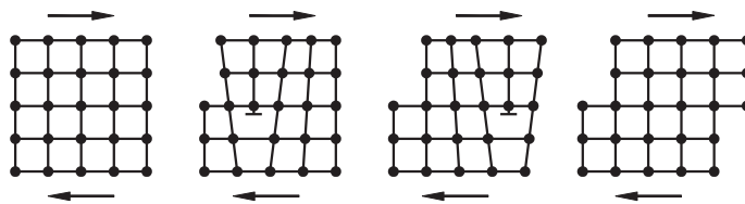
Figure 4.1: Slip displacement of a dislocation [48].
