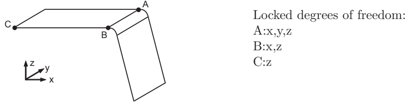
Figure 8.44: Bending experiment; Support conditions for the springback simulation.
