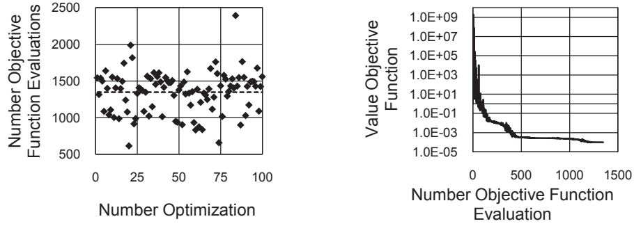
Figure 7.6: This investigation is based on the (1 + 1) -CMA-ES algorithm and the AAOMAC is applied; Left: Analysis of the number of the needed objective function evaluations for finding the optimum; Right: Propagation of a single optimization (Optimization 30).
