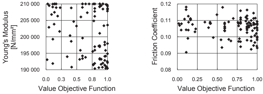
Figure 8.12: YLIT-4-BMW; Left: Relation between the Young's modulus and the objective function; Right: Relation between the friction coefficient and the objective function.
