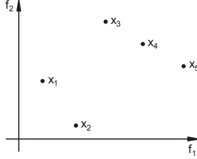
Figure 2.1: Example of non-dominated and dominated solutions.
