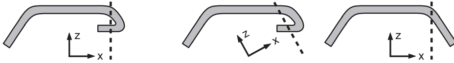
Figure 3.8: Example; Left: Analysis of the undercut of the part geometry with respect to direction 1. The part geometry possesses a zone of undercut with respect to the selected direction; Middle: Analysis of the undercut of the part geometry with respect to direction 2. The shown modification of the part alignment also leads to a zone of undercut; Right: Analysis of the undercut with respect to the intermediate geometry. This geometry in combination with the selected drawing direction does not show any undercut but needs an additional forming step.
