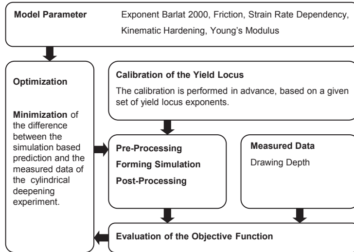
Figure 9.9: Cylindrical deepening experiment; Sequence of the optimization.
