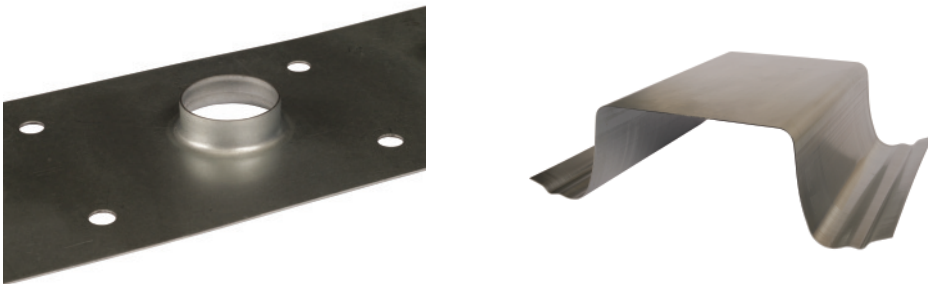
Figure A.4: Left: Hole extrusion experiment; The shape of the specimen after the forming operation; Right: U-Profile experiment; The shape of the specimen after the forming operation.
