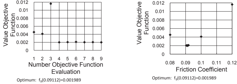
Figure 8.36: Friction experiment; Lagrange interpolation; Left: Propagation of the optimization; Right: Relation between the friction coefficient and the objective function.
