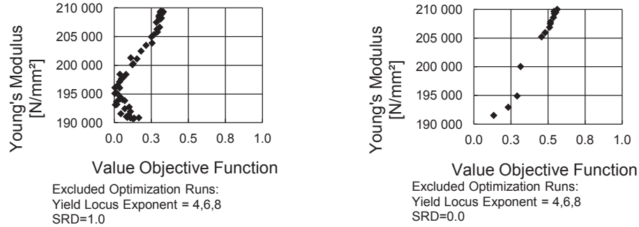
Figure 8.27: Bending experiment; Analysis of the Young's modulus based on a yield locus exponent equal to 5; Left: Objective function evaluations without consideration of the strain rate dependency of the hardening effect; Right: Objective function evaluations with consideration of the strain rate dependency of the hardening effect.
