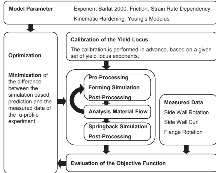
Figure 9.2: U-Profile experiment; Sequence of the optimization.
