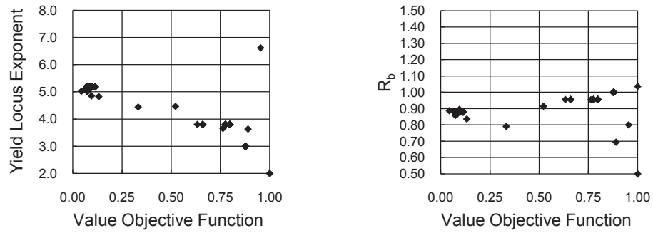
Figure 8.20: YLIT-4-BMW; SQP; Left: Relation between the yield locus exponent and the objective function; Right: Relation between the R_b value and the objective function.
