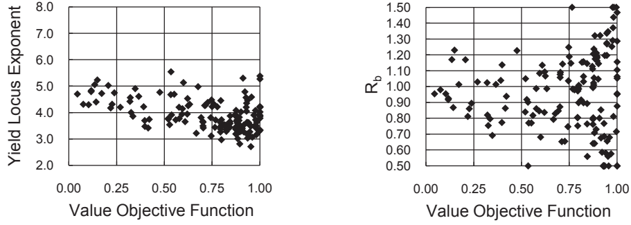
Figure 8.16: YLIT-4-BMW; (\mu/\mu, \lambda) -CMA-ES; Left: Relation between the yield locus exponent and the objective function value; Right: Relation between the R_b value and the objective function.
