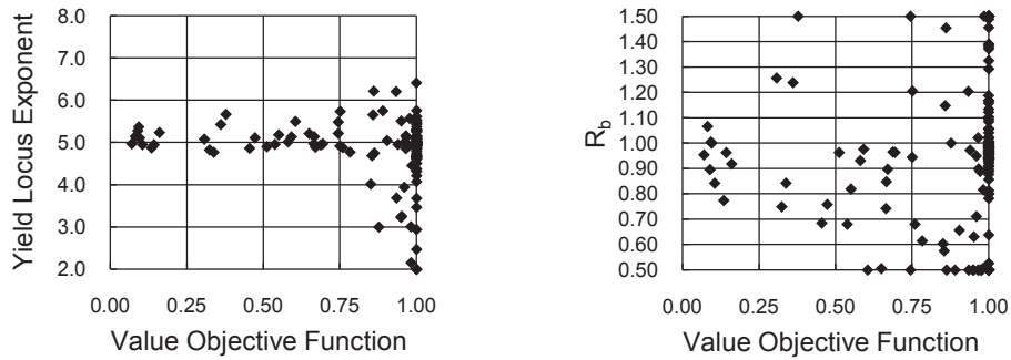
Figure 8.18: YLIT-4-BMW; (1 + 1) -CMA-ES; Left: Relation between the yield locus exponent and the objective function; Right: Relation between R_b value and the objective function.
