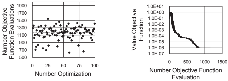
Figure 7.7: This investigation is based on the (1 + 1) -CMA-ES algorithm and the MAHDF is applied; Left: Analysis of the number of the needed objective function evaluations for finding the optimum; Right: Propagation of a single optimization (Optimization 93).
