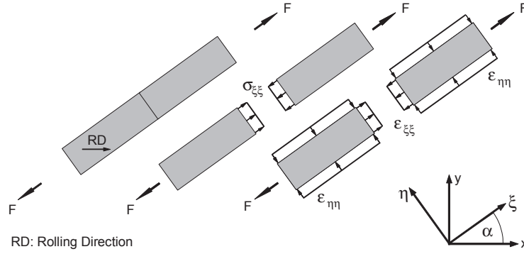
Figure 7.1: Tensile test; Stress state in the \xi, \eta -plane.
