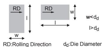
Figure 6.9: YLIT-Experiments; Specimens of the experiments.
