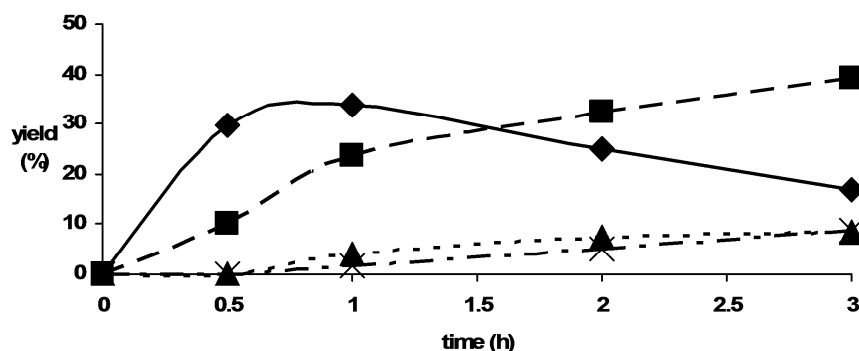
Figure 2.2. Formation of phenol-derived products in the reaction of 4- tert -butylphenol with allyl alcohol in time in a typical experiment; ( \blacklozenge ) 3 ( \blacksquare ) 4 ( \blacktriangle ) 5 ( \times ) 6 . Reaction conditions: ratio 4- tert -butylphenol/allyl alcohol/[RuCp( o -EtOdppe)]/AgOTs = 1000/1000/1/2, toluene, 100 °C. 5 mmol of phenol was used.
