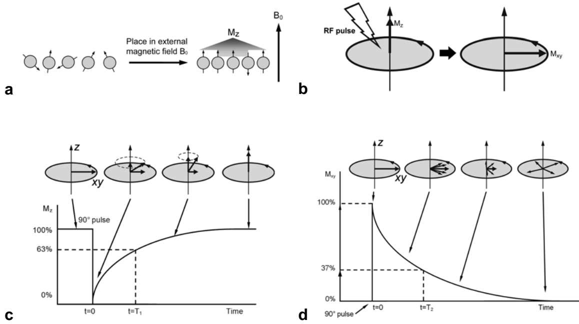
Figure 2.1: MR basics. (a) Protons ( ^1\text{H} ) possess a magnetic moment, or “spin”. When placed in an external field B_0 , the majority of these spins align parallel to B_0 (along the z -axis), resulting in a magnetization vector M_z . (b) Application of a 90^\circ RF pulse flips M_z into the xy -plane (perpendicular to B_0 ), resulting in magnetization vector M_{xy} and phase coherence between spins. (c) M_z will return to its original distribution along the z -axis through T_1 relaxation (eq. 2.3). (d) Loss of phase coherence, and thereby loss of magnetization in the xy -plane, is determined by T_2 relaxation (eq. 2.4).
