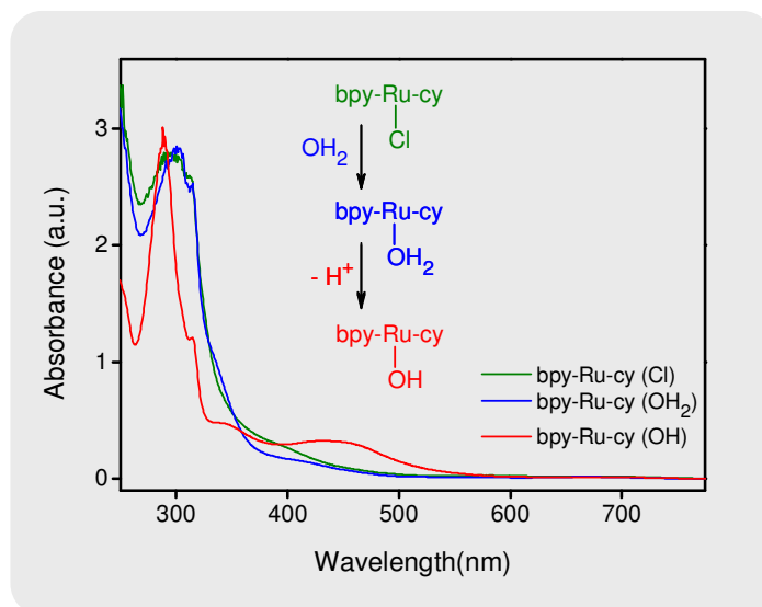
Figure 3.2. Electronic absorption spectra of the [(bpy)Ru(cy)-(Cl)]^+ complex (green line) following blue curve attributed to the formation of [(bpy)Ru(cy)-(OH_2)]^{2+} catalyst induced by aqua exchange and deprotonation of the aqua [(bpy)Ru(cy)-(OH_2)]^{2+} complex to form [(bpy)Ru(cy)-(OH)]^+ (red line). For all measurements a concentration of the complex of 7.5 \times 10^{-5} M was used.
