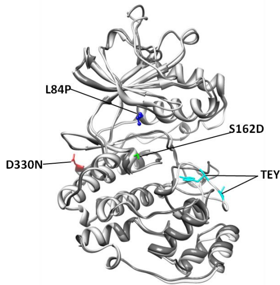
Fig1: Overlap of homology predicted protein models showing the active (grey) and inactive (white) zebrafish ERK2 protein structure . Phosphorylation of the dual phosphorylation site (TEY) causes structural rearrangement of the activation lip. The substitutions may cause rearrangements of intermolecular interactions between amino acids resulting in a smaller distance between the activation lip with the TEY motif and the catalytic site and facilitating autophosphorylation. The L83P site (blue) is located in \alpha -helix C and S162D (green) in the catalytic loop, both in the active site of the kinase. The D330N (red) mutation is located in the CD-site which is a docking site for inhibitory phosphatases. The D330N substitution prevents ERK inhibitory phosphatases to bind. The atomic resolution models of zebrafish ERK2 were constructed with the zERK2 amino acid sequence (ENSEMBLE:ENSDARP00000038550) and based on three dimensional X-ray crystallography predictions PDB:1ERK and PDB:2ERK (phosphorylated). Homology modelling was performed using free online Swiss-model and models were illustrated with Chimera.
