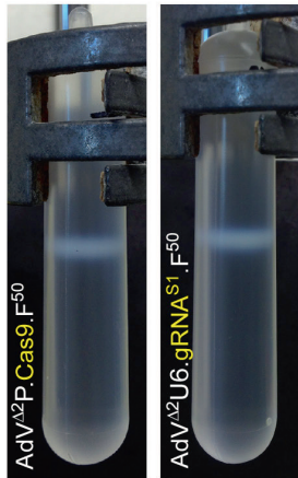
Figure 3. Structural analysis of AdV genomes. (A) Genome-containing AdV particles after ultracentrifugation banding through continuous CsCl density gradients (B) Characterization by restriction fragment length analysis of DNA isolated from CsCl-purified AdV particles. Left panels, in-gel and in silico restriction patterns of AdV Δ2P .Cas9.F 50 genomes (lanes 1) and respective pAdV Δ2P PGK.Cas9.F 50 parental plasmid (lanes 2) treated with BglII. Right panel, in-gel and in silico restriction patterns of AdV Δ2U6 .gRNA S1 .F 50 DNA (lanes 3) and corresponding pAdV Δ2U6 .sgRNA S1 .F 50 parental plasmid (lanes 4) digested with Bsp1407I. Lanes M, GeneRuler DNA Ladder marker.
