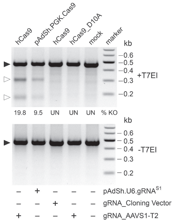
Figure 2. Transient transfection experiments for validating AdV shuttle plasmids pAdSh.PGK.Cas9 and pAdSh.U6.gRNA S1 . AAVS1-specific PCR products amplified from E1-transformed PER.C6 cells co-transfected with hCas9 (9.6 kb) and gRNA_AAVS1-T2 (4 kb), pAdSh.PGK.Cas9 (11.6 kb) and pAdSh.U6.gRNA S1 (7.3 kb), hCas9 and “empty gRNA” construct gRNA_Cloning Vector (3.9 kb), hCas9_D10A (9.6 kb) and gRNA_AAVS1-T2 or mock-transfected. Marker, Gene Ruler DNA Ladder (Fermentas). Plasmids hCas9 and hCas9_D10A express Cas9 nucleases which induce a DSB and a nick at AAVS1, respectively. After amplicon denaturation and reannealing, the presence of mismatches derived from NHEJ-mediated repair of site-specific DSBs in cellula was probed by T7 endonuclease I (T7EI) digestions (upper panel). Negative controls were provided by amplicons not exposed to T7EI (-T7EI) as well as T7EI-treated amplicons (+T7EI) corresponding to mock-transfected cells, to cells co-transfected with hCas9 and gRNA_Cloning Vector and to cells co-transfected with hCas9_D10A and gRNA_AAVS1-T2 encoding the “nickase” mutant version of Cas9 (i.e. Cas9 D10A ) and gRNA S1 , respectively. Solid and open arrowheads indicate the positions of, respectively, undigested and T7EI-digested DNA fragments whose sizes are consistent with DSB formation at the AAVS1 target site. % KO and UN, knockout frequency and undetected, respectively.
