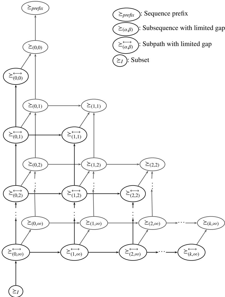
Figure 3.3: A visualization of the relations between several sequence orders. An edge from R_1 to R_2 denotes that R_1 is more general than R_2 , R_1 \geq' R_2 . Only edges which do not follow from transitivity are shown.
