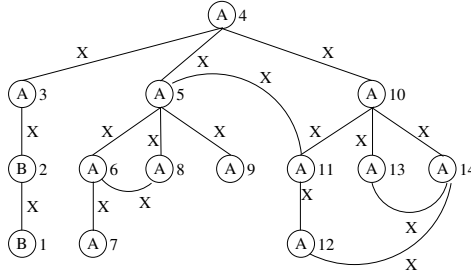
Figure 6.7: A cyclic graph, depicted such that its canonical depth sequence is easily recognizable. The nodes are numbered in the order in which they occur in an edge sequence.
