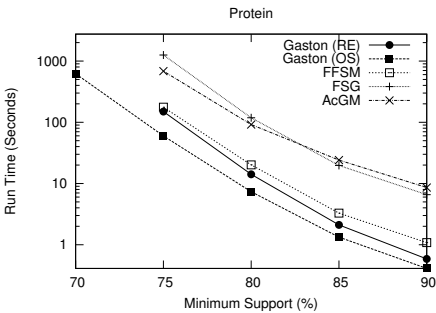
Figure 6.13: Run time experiment on the Protein dataset.
