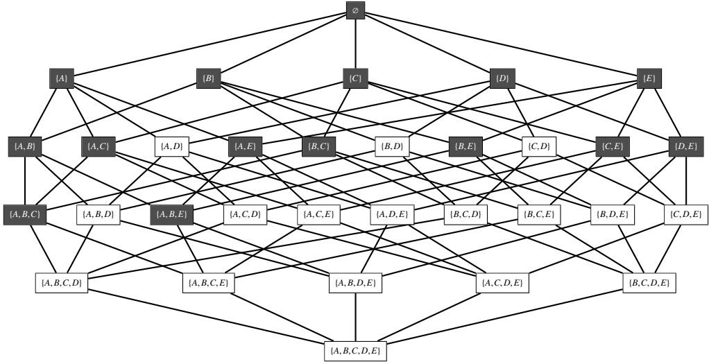
Figure 2.2: A visualization of the search space for the database of Figure 2.1; frequent items for \text{minsup} = 2 are highlighted.
