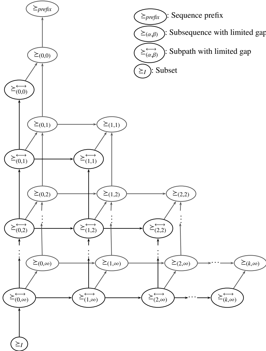
Figure 3.3: A visualization of the relations between several sequence orders. An edge from R_1 to R_2 denotes that R_1 is more general than R_2 , R_1 \succeq' R_2 . Only edges which do not follow from transitivity are shown.
