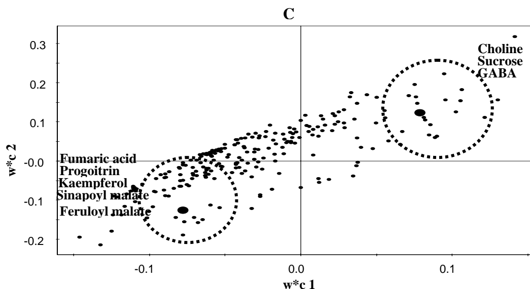
Figure 4.2. The score plot of PCA (PC1 vs. PC2) of control and infected plants ( A ), the score plot of PLS-DA (PLS-component 1 vs. PLS-component 2) of control and infected plants ( B ) and the loading score plot of PLS-component 1 vs. PLS-component 2 ( C ). Rc: Raapstelen control, Ra: Raapstelen infected with Aspergillus niger , Rl: Raapstelen infected with Leptosphaeria maculans , Rf: Raapstelen infected with Fusarium oxysporum , Hc: Herfstraap control, Ha: Herfstraap infected with Aspergillus niger , Hl: Herfstraap infected with Leptosphaeria maculans , Hf: Herfstraap infected with Fusarium oxysporum , Oc: Oleifera control, Oa: Oleifera infected with Aspergillus niger , Ol: Oleifera infected with Leptosphaeria maculans , Of: Oleifera infected with Fusarium oxysporum .
