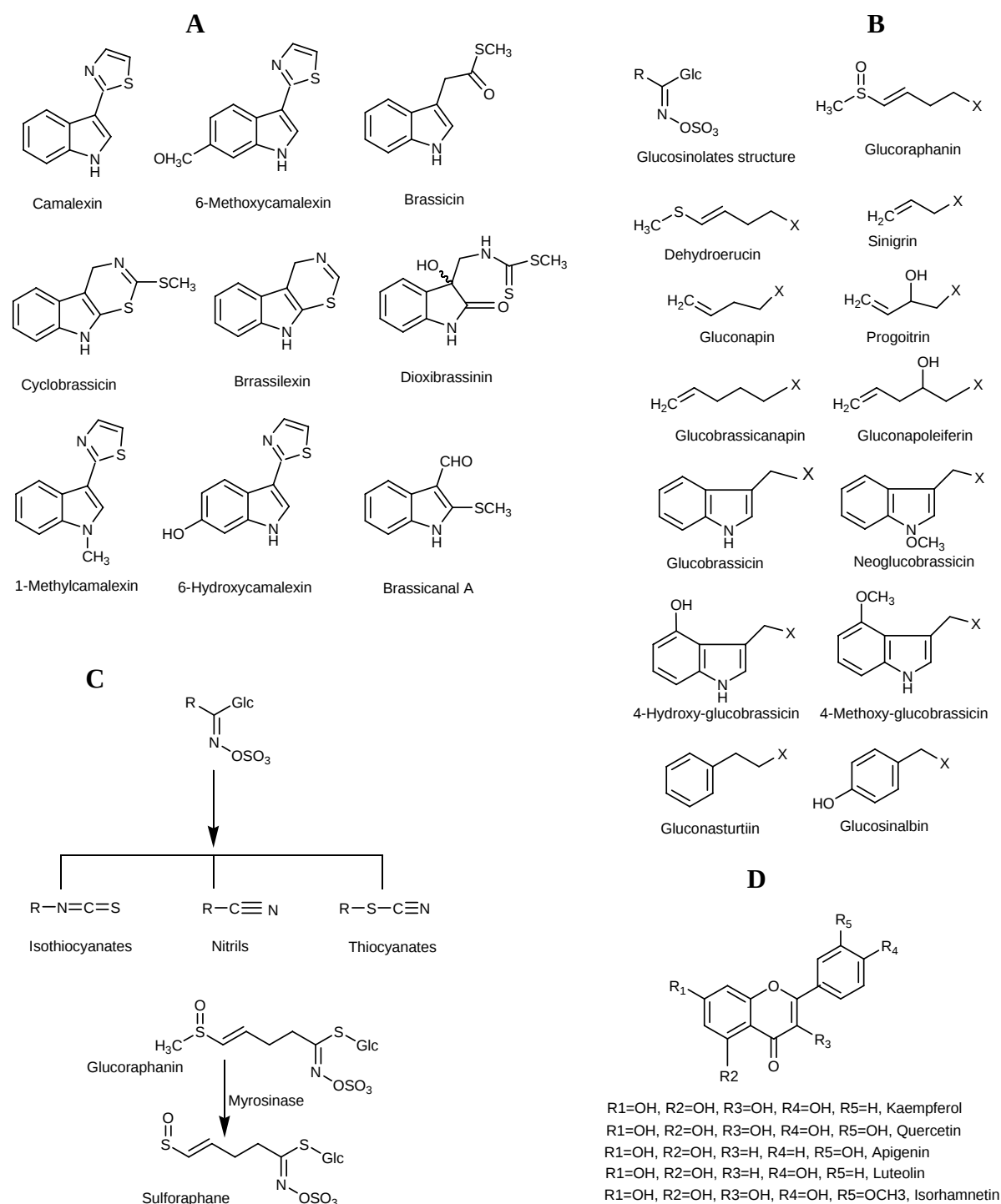
Figure 2.1. Chemical structures of some antifungal secondary metabolites in Brassicaceae, A: Phytoalexins, B: Glucosinolates, C: Glucosinolates hydrolysis by myrosinase enzyme, D: Flavonoids.
