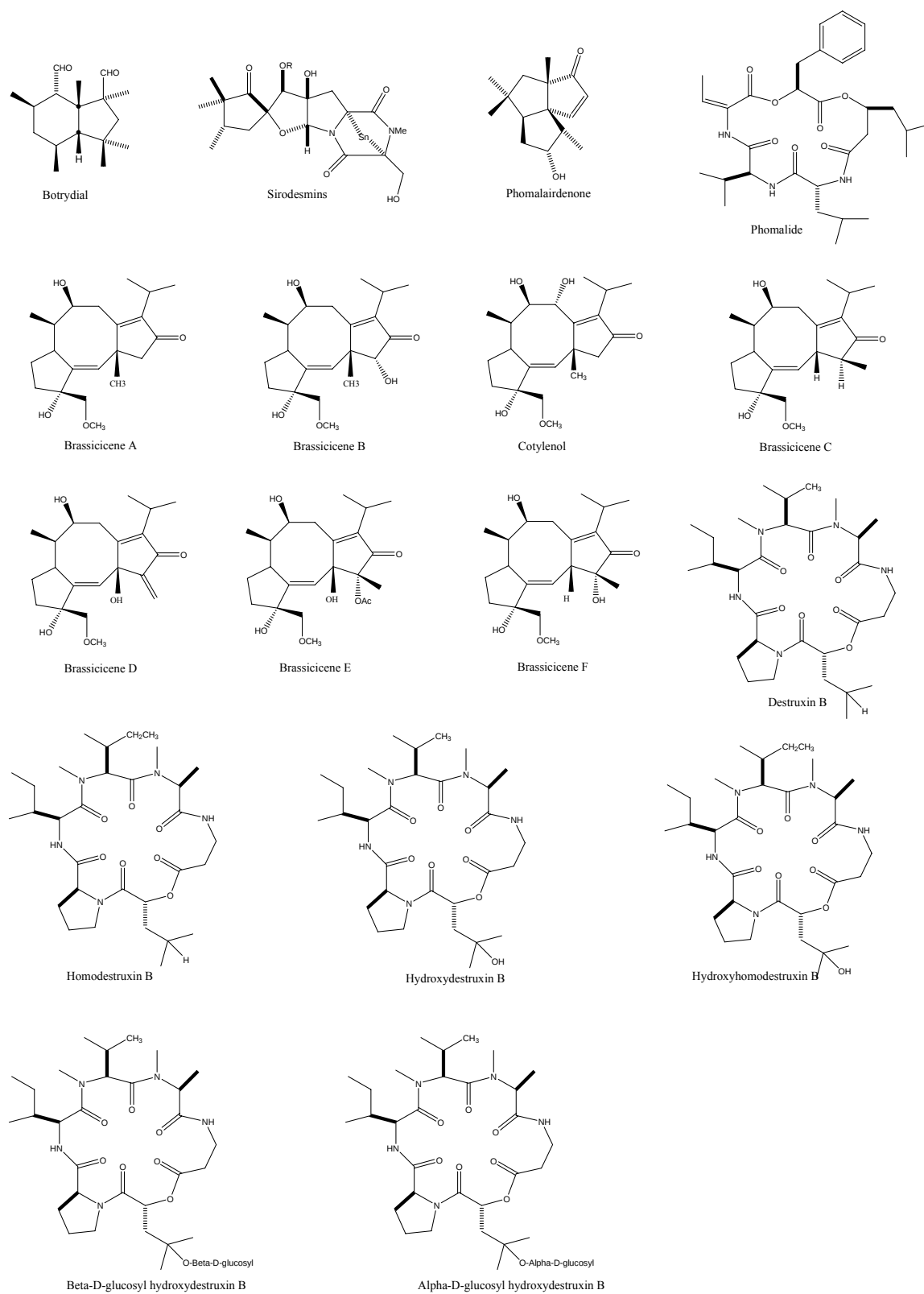
Figure 2.3. Chemical structures of some host-selective toxins and secondary metabolites of some crucifer infected fungi.
