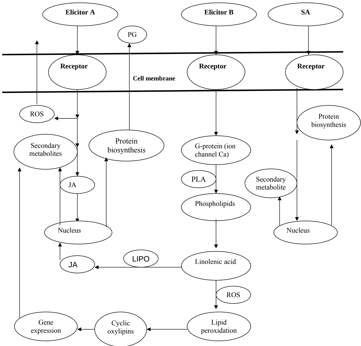
Figure 2.2. Scheme for biosynthesis of defensive secondary metabolites in plants, LIPO: lipoxygenase, PG: polygalacturonase, PLA: phospholipase A, ROS: reactive oxygen species, SA: salicylic acid, JA: jasmonic acid.
