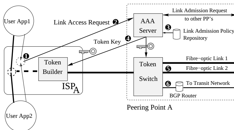
Figure 8.2: Token based networking architecture.
