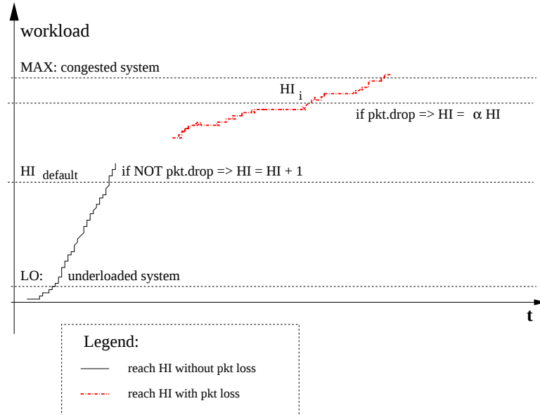
Figure 7.6: AIMD control behaviour.
