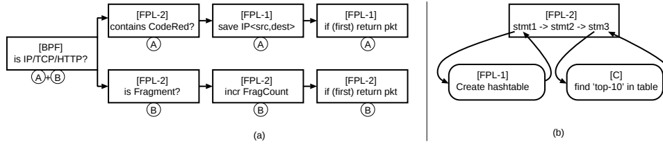
Figure 2.2: (a) combining different languages in two flows (A and B), (b) calling external functions from a single flow
