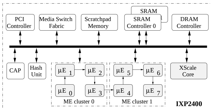
Figure 2.5: The IXP2400 NP block diagram.
