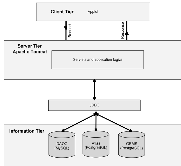
Figure 2: The 3 tier architecture of the 3D-VisQus.
