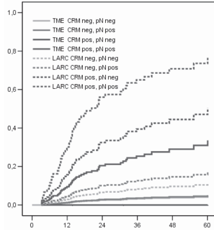
Figure 4b. Cox regression: local recurrence, categorized in treatment, margin and lymphnodes
