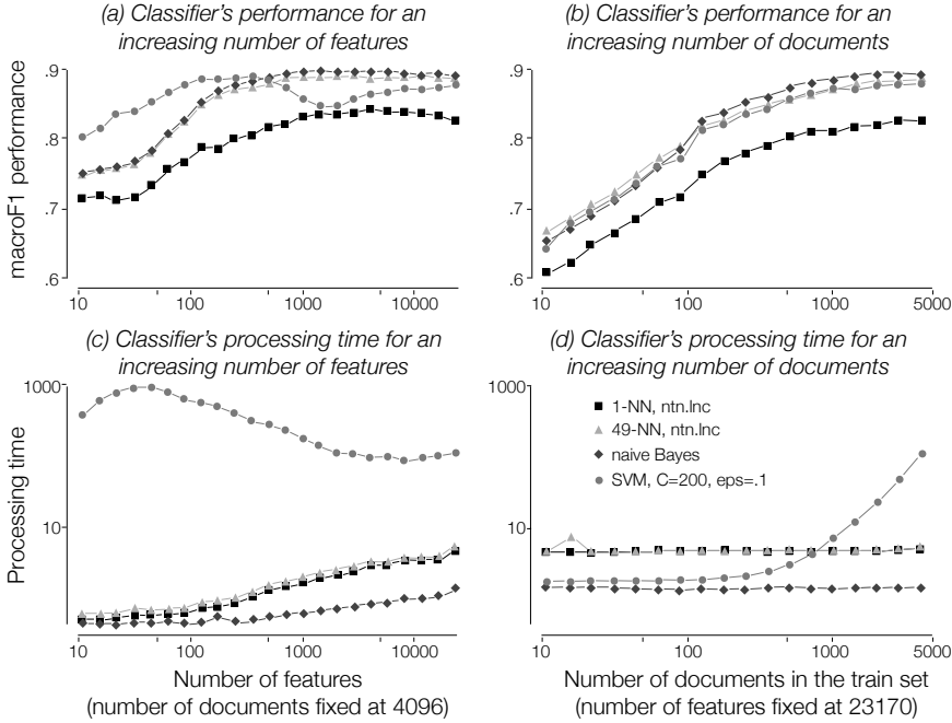
Figure 7.3: Classifier's performance (a, b) and processing time (c, d) on C01-C21 (Ohsumed-All) given an increasing number of features (a, c) and of documents (b, d).
