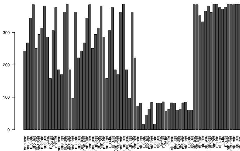
Figure B.3: Counts of pairwise wins for each transformation, from nnc.anc to ntn.ntn .
