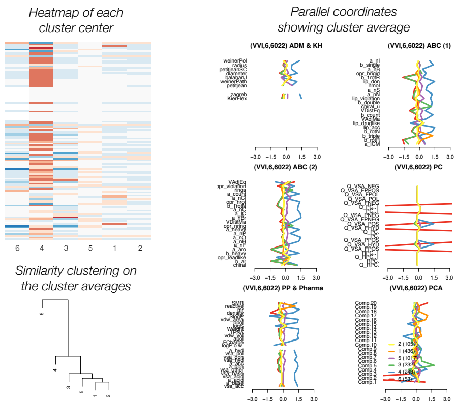
Figure 4.3: This Figure illustrates the six average patterns of (VVI, 6, 6022). It also characterizes the different subtypes on all variables grouped by factors. The scales on the parallel coordinate plots refer to the z-scores with 95% of the values that should fit within [-2, 2] . In this Figure, the blue subtype with (248) molecules displays an especially high profile for most descriptors, the red (53) and green (232) subtypes show comparatively low profiles. In particular, these two subtypes differ on the partial charge descriptors (PC). We may account the "zigzag" of the red subtype to the numerical type of these variables which are counts.
