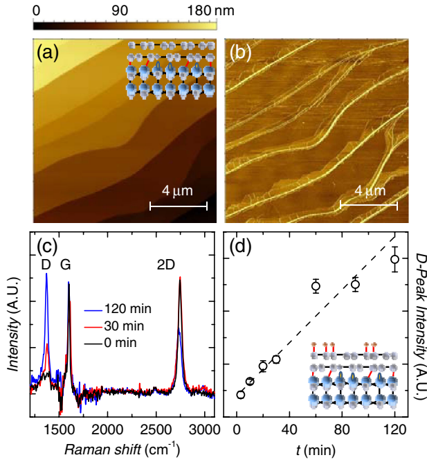
FIG. 1 (color online). (a) Atomic force micrograph of the typical SiC terrace structure on top of which the graphene is grown. The inset shows a schematic of the surface structure with from top to bottom a graphene layer, a buffer layer, and the SiC substrate. The gray spheres represent carbon, the blue spheres silicon, and the yellow ovals the silicon dangling bonds. (b) Phase image showing the single layer graphene areas on top of the terraces and the narrow bilayer regions at the terrace edges. (c) Raman spectra of hydrogenated graphene with a treatment time t = 0 min. (black), 30 min. (red), and 120 min. (blue). Clearly visible is the upcoming D -peak intensity with increasing treatment time. (d) D -peak intensity as a function of treatment time (the line is a guide to the eye). The inset shows the schematic bonding of hydrogen (orange spheres) to the graphene layer.
