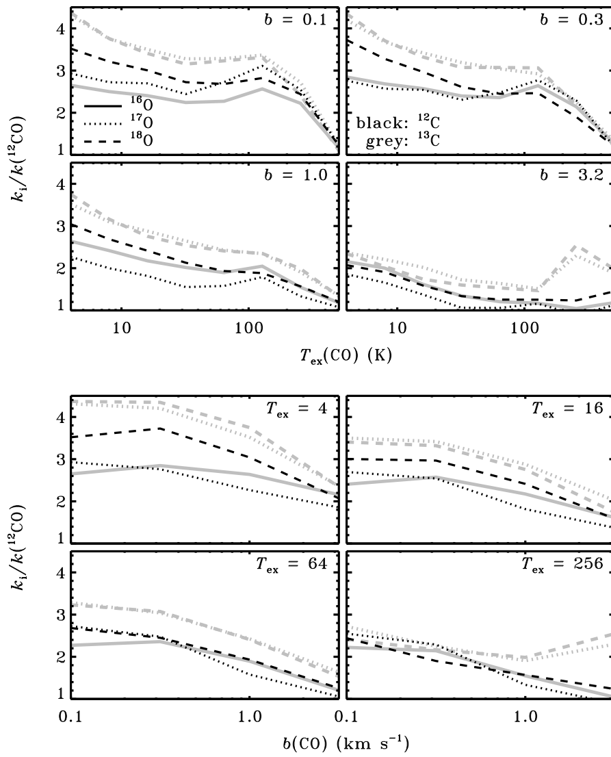
Figure 5.5 – As Fig. 5.4, but with all rates normalised to the 12 CO rate.
