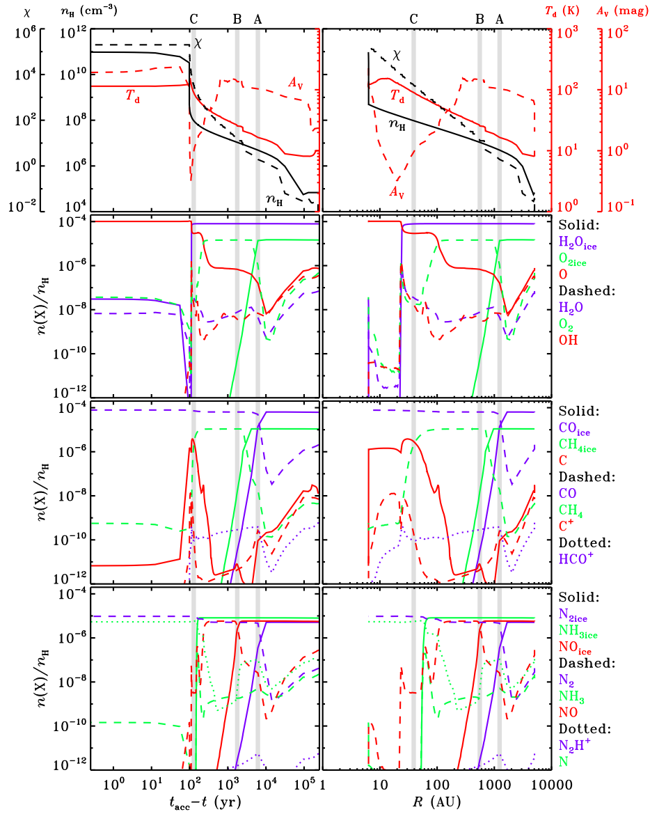
Figure 3.2 – Physical conditions ( \chi , n_H , T_d and A_V ) and abundances of the main oxygen-, carbon- and nitrogen-bearing species for the single parcel from Sect. 3.5.1, as function of time before the end of the collapse (left) and as function of horizontal position (right). The grey bars correspond to the points A, B and C from Fig. 3.3. Note that in each panel, the parcel moves from right to left.
