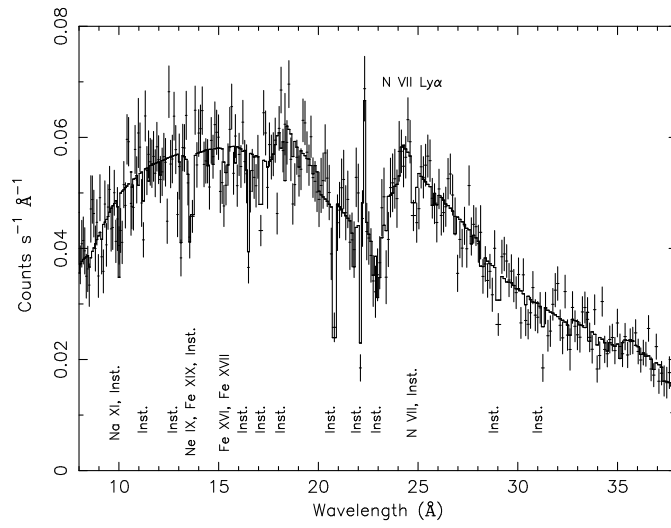
Figure 3.6: Fit to the RGS data with model 6 of Table 3.4. For clarity RGS 1 and RGS 2 were binned by a factor of 10 and added. The relativistic N VII Ly \alpha line is indicated by N VII Ly \alpha written horizontally. The features labeled Inst. are periodic dips due to CCD-gaps, or due to instrumental calibration.
