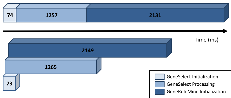
Figure 4.4: Benchmark comparison with a t-score threshold of 15
