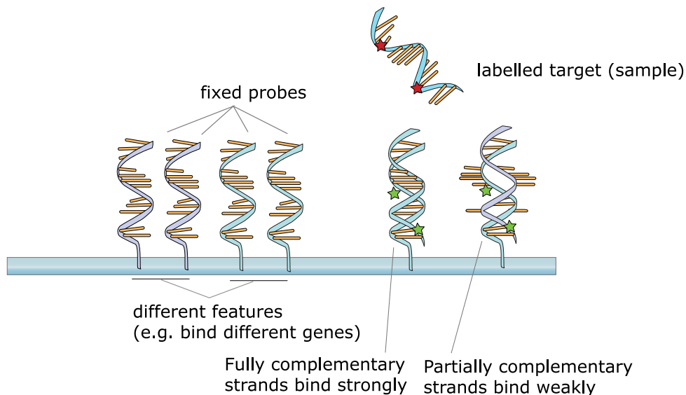
Figure 7.3: Microarray hybridization
