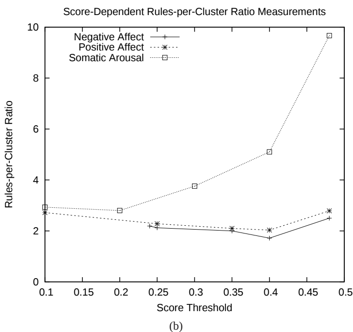
Figure 8.10: Cluster ratio measurements of the ontology mappings experiment
