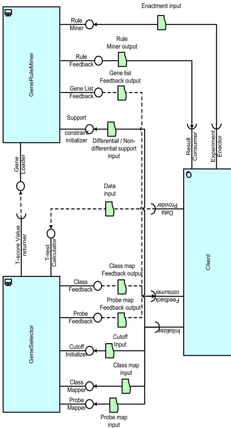
Figure 4.2: The SOKD use case design
