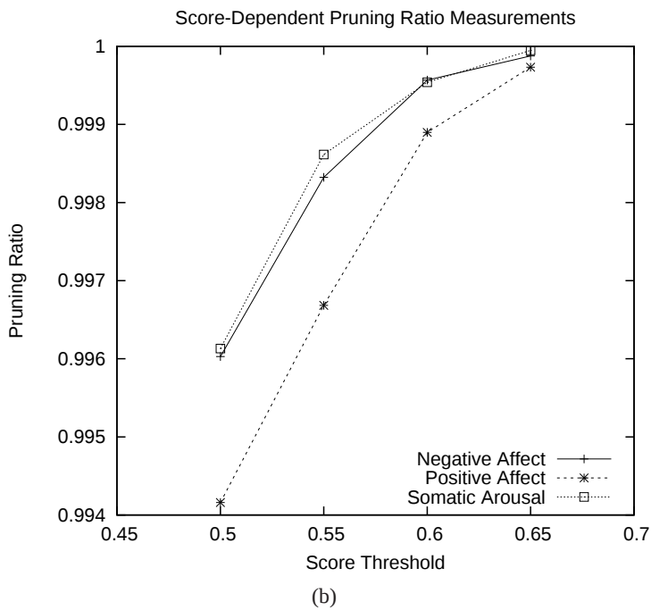
Figure 8.4: Pruning ratio measurements for the experiments on gene translations
