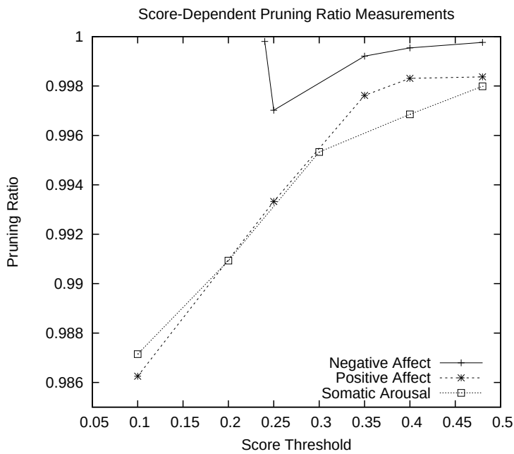
Figure 8.9: Pruning measurements of the ontology mappings experiment
