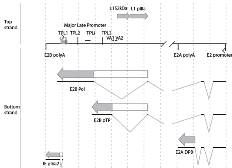
Figure 4. Schematic presentation of genes and regulatory sequences located in the E2 transcription unit. The arrows point in the direction of transcription. Gray arrows depict coding regions while the open white region depicts intron sequences.
