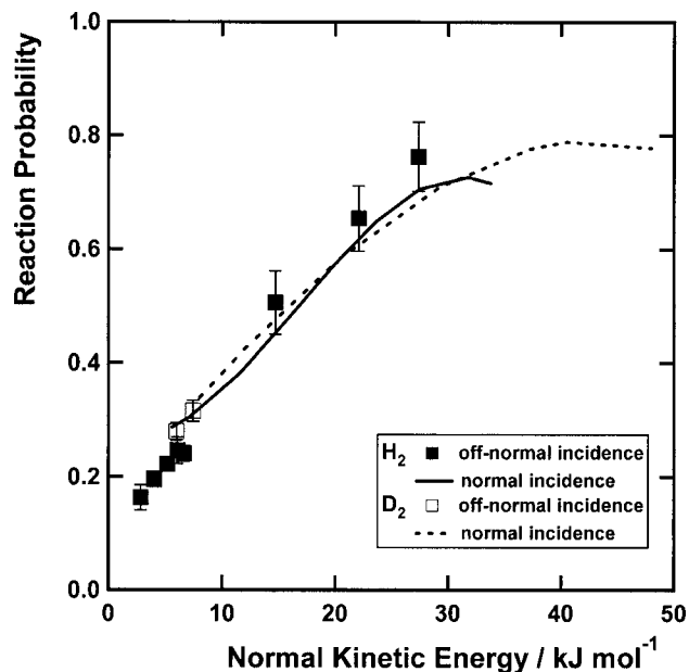
FIG. 2. Comparison of the reaction probabilities of H 2 and D 2 colliding at off-normal incidence (points) and normal incidence (lines).
