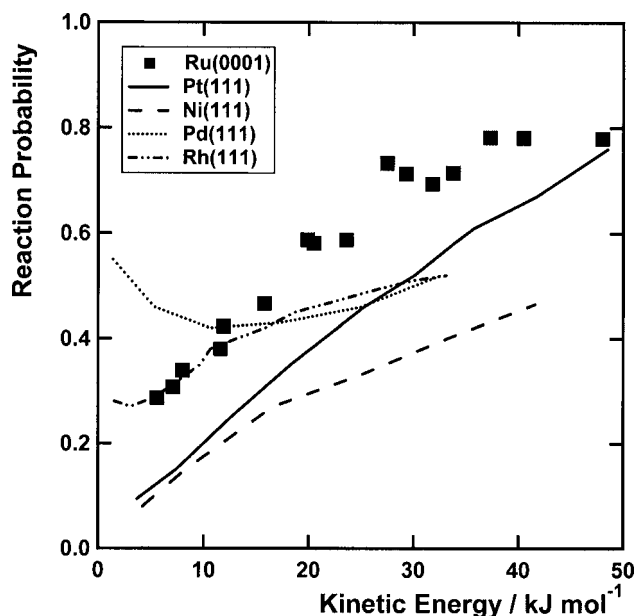
FIG. 3. Comparison of the reaction probabilities of \text{H}_2 and \text{D}_2 for various metals.
