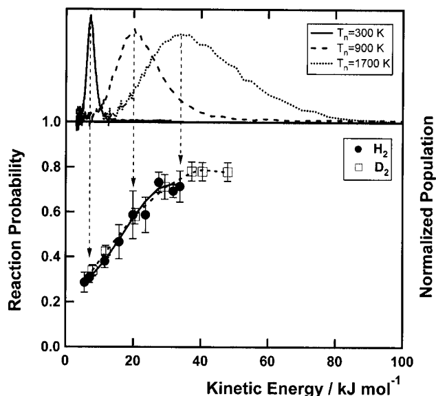
FIG. 1. Lower panel: Reaction probability of hydrogen on Ru(0001) at normal incidence. Data are fitted with fourth-order polynomials. Top panel: Convoluted energy distributions for various nozzle temperatures (see text for details).
