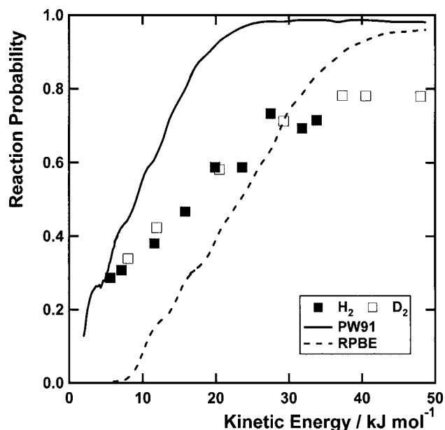
FIG. 4. Comparison of experimental data with predictions from a theoretical study using two different functionals (Ref. 14).
