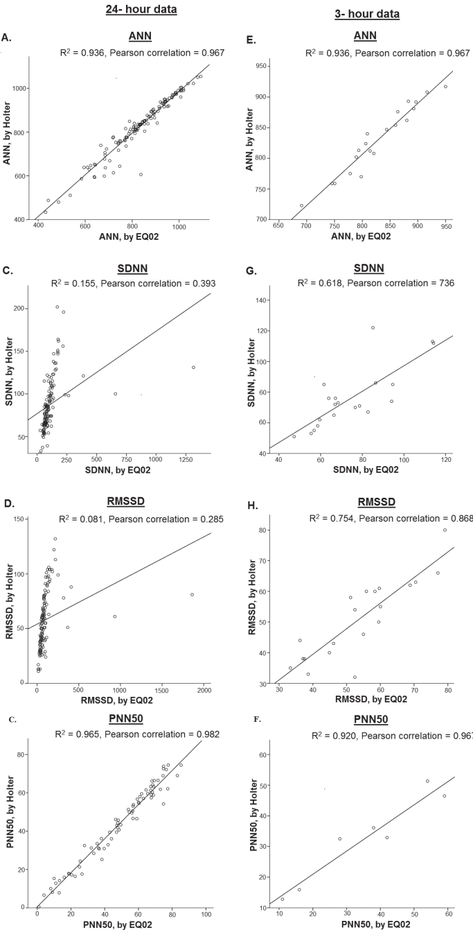
FIGURE 10.8 | Comparison between HRV parameters measured by EQ02 and Holter. Correlation between ANN, SDNN, RMSSD and pNN50 in a participant from both devised over 24hr (A,B, C, D) and in a sub- selection of 3-hour data with artefact percentage 1.15% (E, F, G and H).
