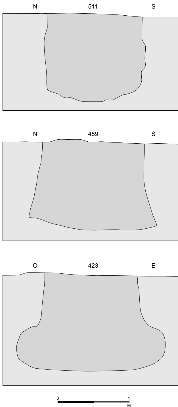
Fig. 2.8 Rémerschen - Schengerwis. Typology of silos: examples of cylindrical, obtuse angled or bell-shaped silos (from De Ruyter/Le Brun-Ricalens 1993) (drawing by Jan Maarten Luursema)
