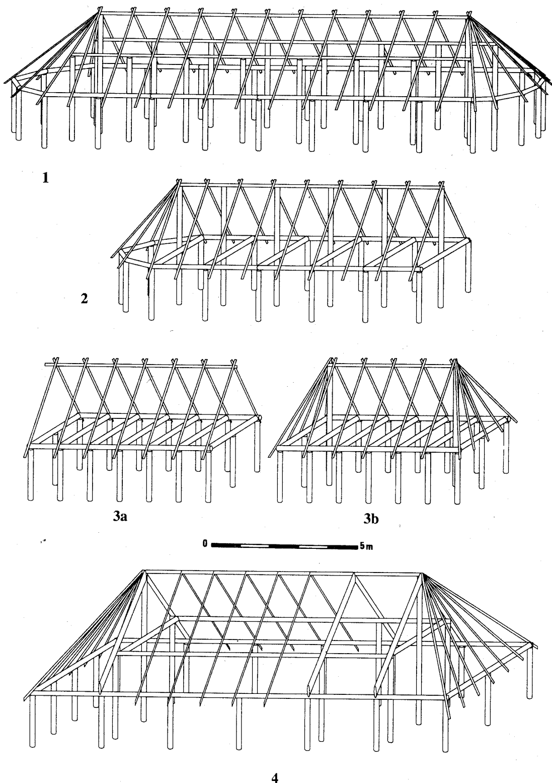
Fig. 2.3 The diachronical development of farmhouse types in the Moselle region in the Bronze Age and the Early Iron Age (from: Blouet et al. 1992). 1= Bronze Ancien, 2= Bronze moyen, 3= Bronze final, 4= Hallstatt Ancien
