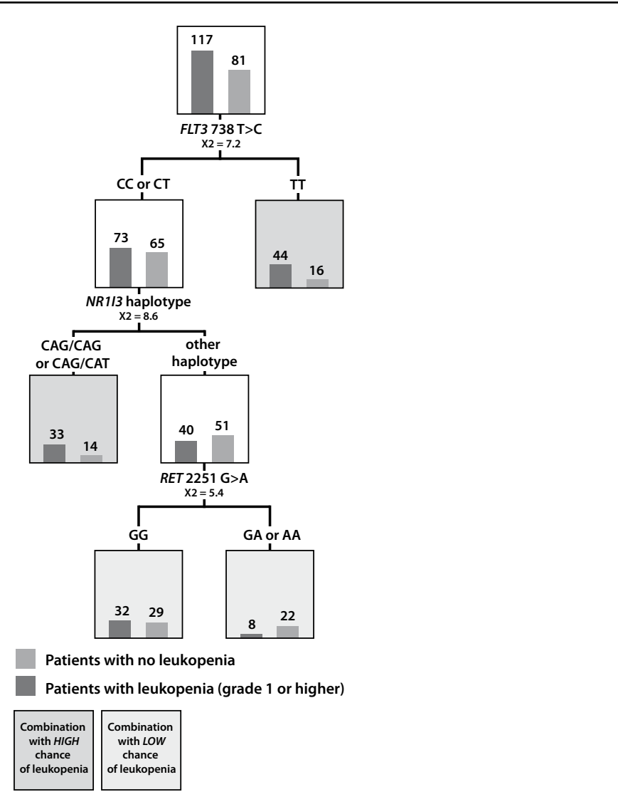
Figure 2 Classification and regression tree analysis of sunitinib-induced leukopenia
