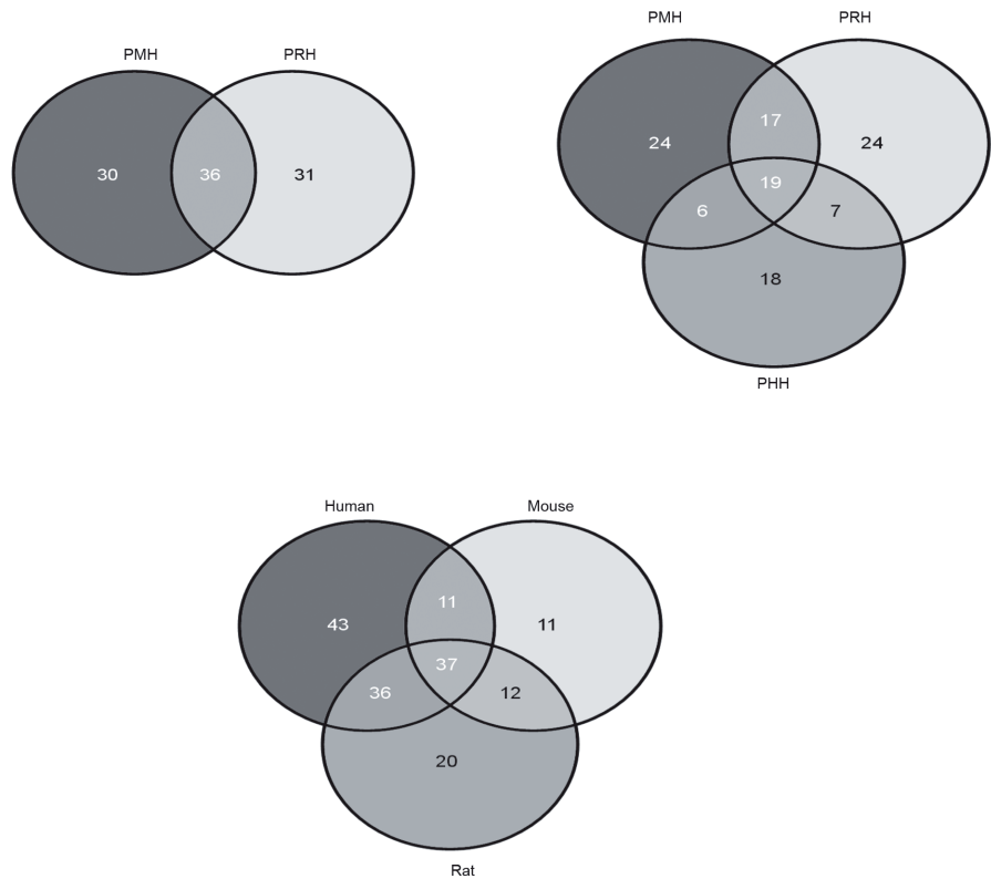
Supplementary S3. Venn diagrams of significantly altered canonical pathways from human, mouse and rat DEG's upon diclofenac exposure.
