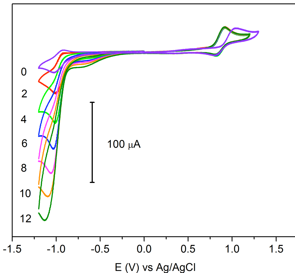
Fig. 5.6. Cyclic voltammograms of [Ni(pbss)Ru(bpy) 2 ](PF 6 ) 2 (0.5 mM) in acetonitrile in the presence of 0–12 equivalents of trifluoroacetic acid. Further details are provided in Table 5.4.
