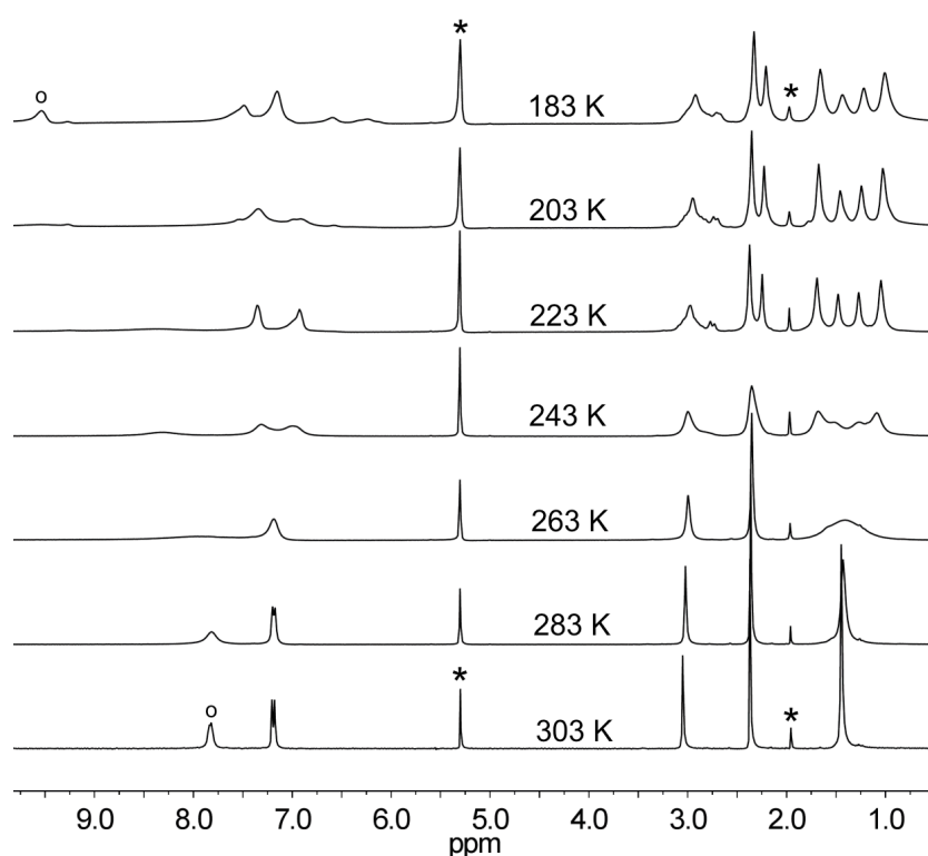
Fig. 7.4. ^1\text{H} NMR of [\{\text{Ni}(\text{mpsms})_2\}_2(\text{CuI})_6] in \text{CD}_2\text{Cl}_2 recorded in different temperatures ranging between 183 and 303 K. ★, signals from \text{CD}_2\text{Cl}_2 (5.32 ppm) and acetone (2 ppm); ○, signals from the ortho -protons of the phenyl rings.
