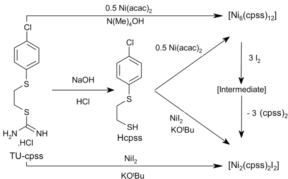
Scheme 6.1. Synthesis of complexes [\text{Ni}_6(\text{cpss})_{12}] and [\text{Ni}_2(\text{cpss})_2\text{I}_2] from TU-cpss, and the chemical oxidation of [\text{Ni}_6(\text{cpss})_{12}] by iodine.
