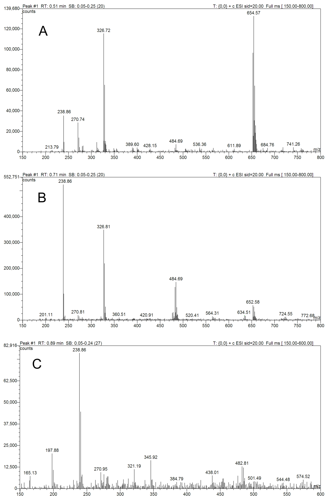
Fig. 8.3. Formation of [\text{Ni}(\text{S}_2\text{S}')_2] from [\text{Ni}(\text{ebsms})_2] , as followed by ESI-MS spectrometry upon irradiation on the toluene solution of [\text{Ni}(\text{ebsms})_2] at room temperature; (A) 0 hrs, (B) 6 hrs, (C) 12 hrs; m/z = 326.72 = [\text{Ni}(\text{ebsms}) + \text{H}]^+ , m/z = 652.57 = [\text{Ni}_2(\text{ebsms})_2 + \text{H}]^+ , m/z = 238.86 = [\text{Ni}(\text{S}_2\text{S}') + \text{H}]^+ .
