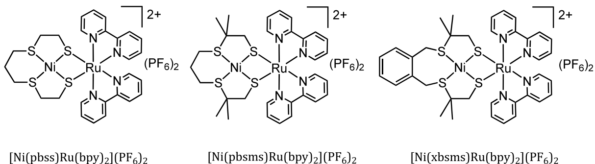
Fig. 5.1 Schematic structures of the heterodinuclear [\text{NiRu}] complexes described in this Chapter.
