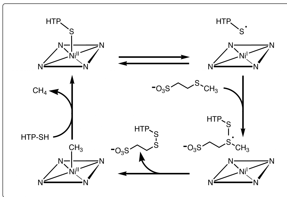
Scheme 1.6. Mechanism of F-430-catalyzed methane formation (Adapted from the literature). 85-87
