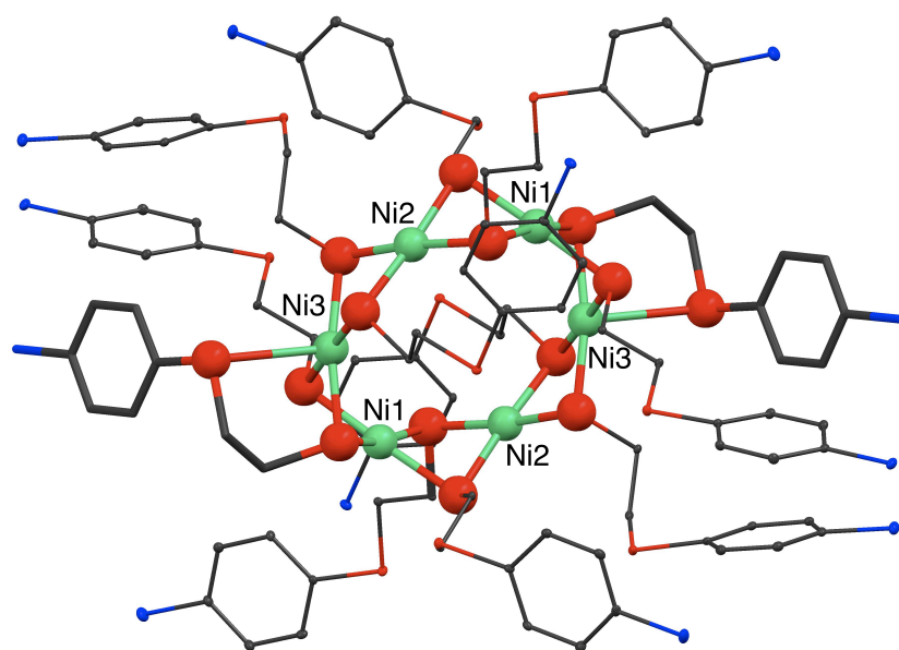
Fig. 6.1. Perspective view of [\text{Ni}_6(\text{cpss})_{12}] . Ni, green; S, red; Cl, blue; C, grey. Hydrogens are omitted for clarity. Symmetry operation a: -x, 1-y, -z . Selected bond lengths (Å): Ni–S, 2.1895(17)–2.2161(16); Ni···Ni, 2.8220(11)–3.1022(12).
