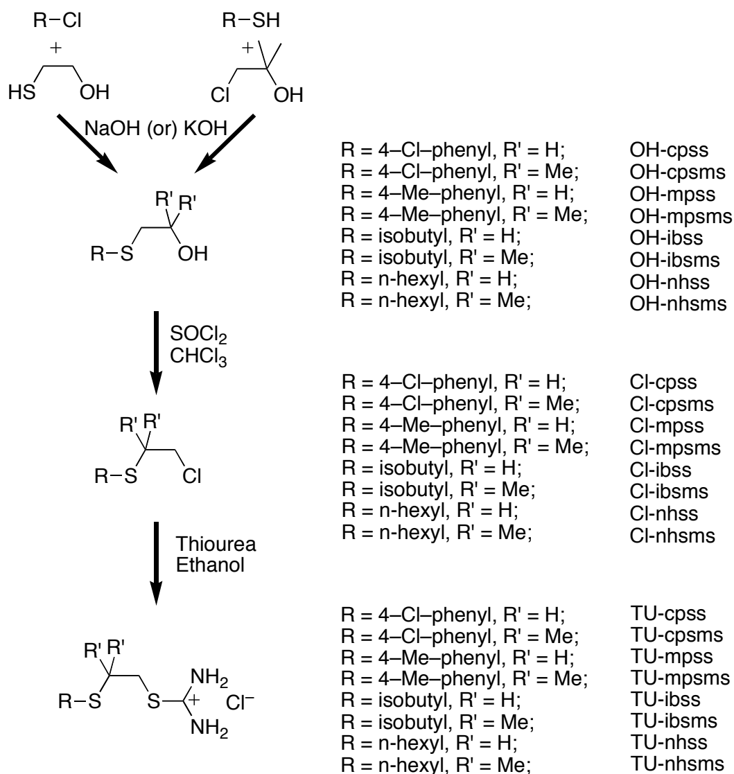
Scheme 2.3. General synthetic route applied for the synthesis of thiouronium salts.
