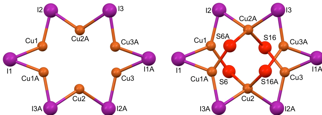
Fig. 7.2. Perspective views of the Cu_6I_6 pucker-crown (left) and Cu_6I_6S_4 cage (right) in [Ni(mpsms)_2]_2(CuI)_6 .
