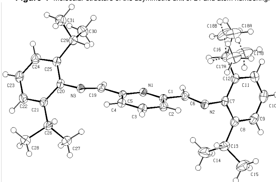
Figure 5 Molecular structure of the asymmetric unit of L2 and atom numbering.
