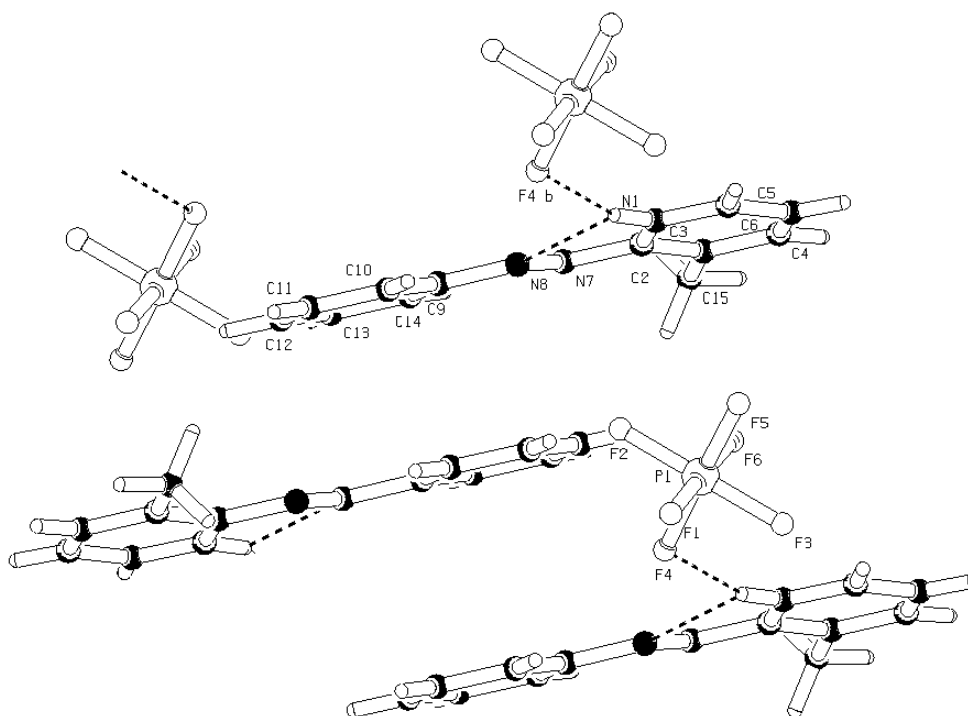
Figure 2 PLATON projection of 3mazpyH showing the cooperative intra and inter hydrogen bonds in the cell unit.
