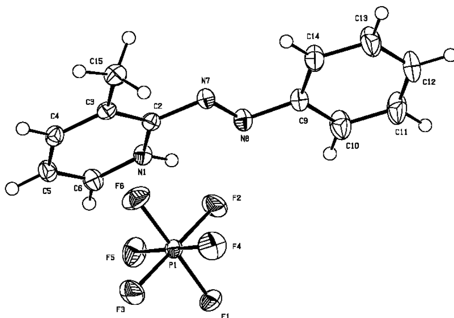
Figure 1 X-ray structure of the asymmetric unit of 3mazpyH with the hexafluoridophosphate anion and used atomic numbering.
