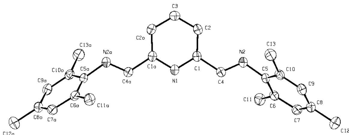
Figure 4 Molecular structure of the asymmetric unit of L1 and atom numbering.
