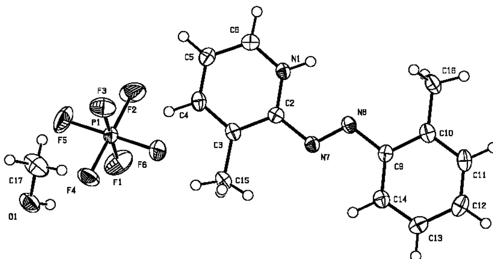
Figure 3 X-ray structure of the asymmetric unit of 3mtazpyH with the hexafluoridophosphate anion and used atom numbering.
