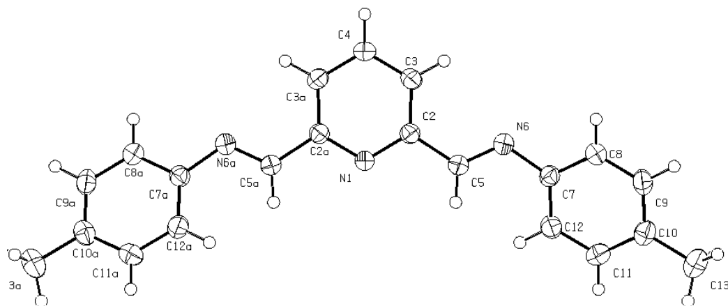
Figure 6 Molecular structure of the asymmetric unit of L3 and atom numbering.
