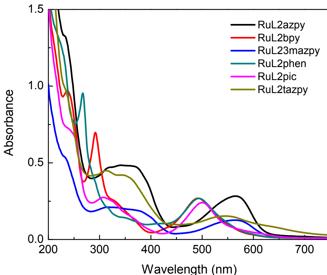
Figure 5.8 Absorption spectra of Ru(II)L2-derivatives in acetonitrile at 294 K.
