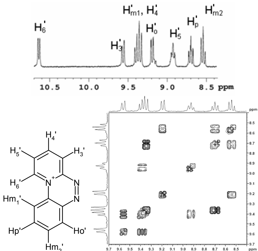
Figure 3.8 1D ^1\text{H} NMR and 2D ^1\text{H} COSY spectra of the pyrium cation in deuterated acetone at 21 ^\circ\text{C} , using TMS as internal standard. Aromatic region only.
