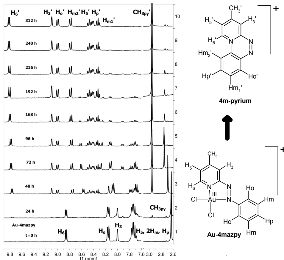
Figure 3.13 Time-dependent ^1\text{H} NMR study of Au-4mazpy in deuterated acetonitrile at 21 °C, using TMS as internal standard. The numbering scheme corresponding to the peak assignments is described in the schematic representation of the new product, the 4m-pyrium cation and the starting material, Au-4mazpy.
