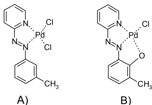
Figure 3.2 Schematic representation of the two products obtained in the synthesis of a palladium compound where the 2-(phenylazo)pyridine metal-mediated hydroxylation is observed [78].
