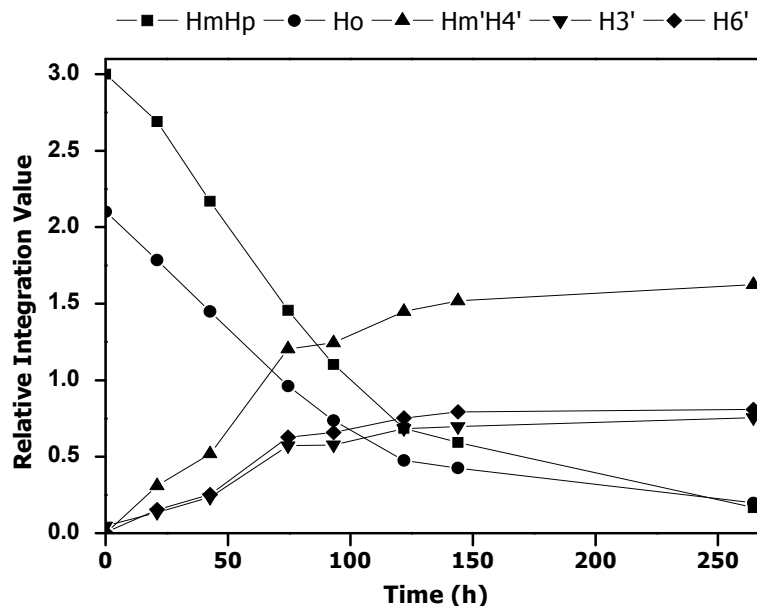
Figure 3.6 Proton resonance peak shifts as a function of time in deuterated acetone solution of Au-azpy at 21 °C. Shifts for new peaks: H 6' , 10.6312; H 3' , 9.5012 and H m' /H 4' , 9.3472.
