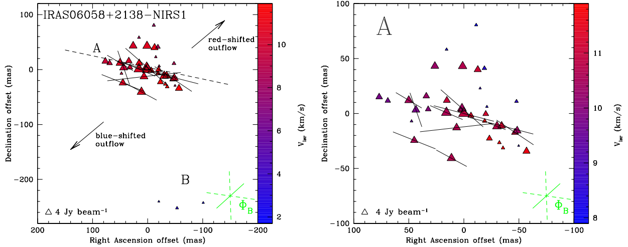
Fig. 2. Left panel: view of the CH 3 OH maser features detected around IRAS 06058+2138-NIRS1 (Table A.1). Triangles symbols identify CH 3 OH maser features scaled logarithmically according to their peak flux density (Table A.1). Maser LSR radial velocities are indicated by color (the assumed velocity of the YSO is V_{\text{LSR}}^{\text{C}^{18}\text{O}} = +3.9 \text{ km s}^{-1} , Saito et al. 2007). A 4 Jy beam -1 symbol is plotted for illustration. The linear polarization vectors, scaled logarithmically according to polarization fraction P_l , are overplotted. On the right-bottom corner the error weighted orientation of the magnetic field ( \Phi_B , see Sect. 6.2.1) is also reported, the two dashed segments indicates the uncertainty. The two arrows indicate the direction of the red- and blue-shifted lobe of the bipolar outflow ( \text{PA}_{\text{out}} = 130^\circ ; Wu et al. 2010). The dashed line is the best linear fit of the CH 3 OH maser features of group A ( \text{PA}_{\text{CH}_3\text{OH}} = 78^\circ \pm 7^\circ ). Right panel: zoom-in view of group A.
