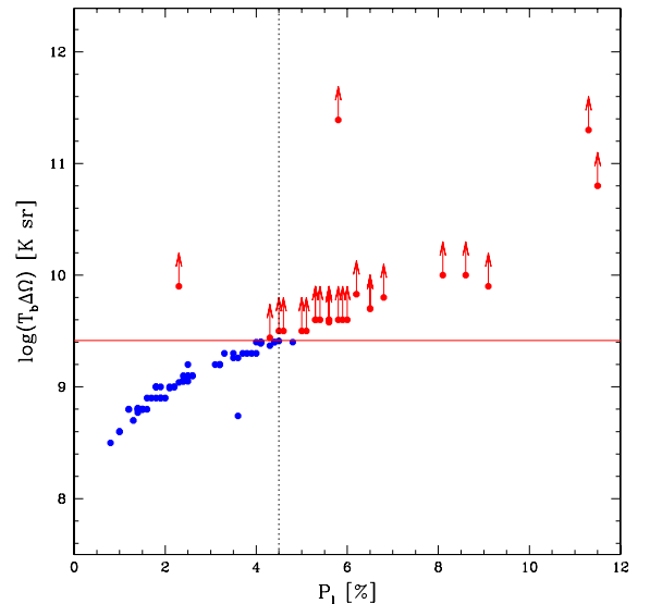
Fig. 6. Emerging brightness temperatures ( T_{\text{b}}\Delta\Omega ) as function of the linear polarization fraction ( P_1 ). The blue and red circles indicate the unsaturated and saturated masers, respectively, detected in NGC 7538 (Surcis et al. 2011a), W51, W48, IRAS 18556+0138, and W3(OH) (Surcis et al. 2012), IRAS 06058+2138-NIRS1, IRAS 22272+6358A, S255-IR, and S231 (this work). The red arrows indicate that the T_{\text{b}}\Delta\Omega values obtained from the adapted FRTM code are lower limits. The red full line is the limit of emerging brightness temperature above which the CH 3 OH masers are considered saturated ( T_{\text{b}}\Delta\Omega > 2.6 \times 10^9 K sr; Surcis et al. 2011a), and the dotted line gives the lower limit to the linear polarization fraction for saturated masers ( P_1 \approx 4.5\% , Surcis et al. 2012).
