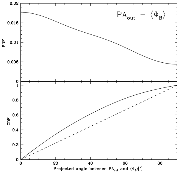
Fig. 8. Probability distribution function (PDF, top panel ) and cumulative distribution function (CDF, bottom panel ) of the projected angle between the magnetic field and the outflow axes ( |PA_{out} - \langle\Phi_B\rangle| ). The dashed line is the CDF for random orientation of outflows and magnetic fields, i.e. all angular differences are equally likely. The results of the Kolmogorov-Smirnov test can be found in Table 3
