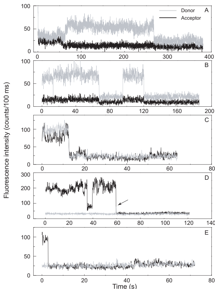
Figure 6.8: Representative fluorescence time traces from frozen dual-labeled polyproline6 molecules. All the traces were recorded by the donor excitation with an integration time of 100 ms and an excitation power of 1 kW/cm 2 except for trace D 2 kW/cm 2 . (A) The two intensities varied in phase in the first 60 s. Then the acceptor intensity went down to the background level and the donor intensity went up to a new level before it was finally bleached. (B & C) The intensities of the donor and acceptor changed in a correlated manner. (D) The donor intensity was on the background level in the first 60 s, whereas the acceptor intensity was relatively high, indicating a high FRET efficiency. However, the acceptor had a period of low emission during which the donor intensity did not recover. When the acceptor was bleached, the donor intensity simultaneously jumped up, indicated by the arrow, but went down to the background level very quickly. (E) The traces showed a high FRET efficiency in the beginning. When the acceptor was bleached, the donor intensity still remained the same.
