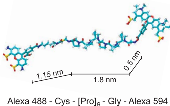
Figure 6.2: Structure of dual-labeled polyproline 6. The contour length of polyproline 6 is about 1.8 nm. The lengths of two linkers are about 1.15 nm and 0.5 nm, respectively. If the molecule is fully stretched, the interdye distance is around 3.45 nm. If the two linkers fold back to the backbone, the interdye distance is approaching to 0.15 nm.
