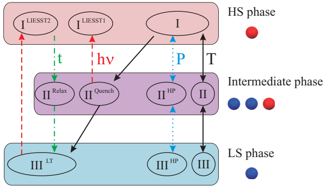
FIG. 2. (Color online) Spin state and transformation pathways between structurally characterized states in 1 . The structural states I, II, and III and the high-pressure \text{II}^{\text{HP}} and \text{III}^{\text{HP}} structural states have been reported in Refs. 40 and 57. The external stimuli triggering the spin state and state changes are temperature (T), pressure (P), and light irradiation ( h\nu ); they are depicted as continuous black, dotted blue, and dashed red arrows, respectively; time evolution (t) is shown as dashed dotted green arrows.
