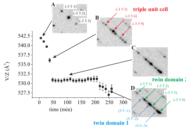
FIG. 6. (Color online) Evolution of the unit cell volume per formula unit ( V/Z ) during the isothermal relaxation at 40 K from the photoinduced metastable state I^{LIESST2} , and selected region of the diffraction pattern centered on the [-3 \ 5 \ l] row.
