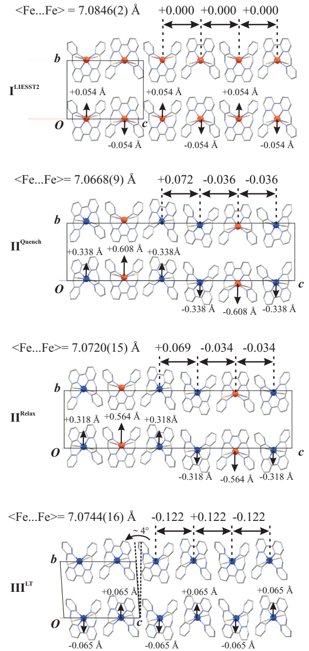
FIG. 3. (Color online) Section of the crystal packing in the (bc) plane indicating the displacement of the \text{Fe}^{II} atoms along the b direction from the regular y = 0 position, and \text{Fe}\dots\text{Fe} separation distances along the c direction with respect to the average \text{Fe}\dots\text{Fe} distance. HS \text{Fe}^{II} centers are shown in red, LS \text{Fe}^{II} centers in blue. Hydrogen atoms have been omitted for clarity.
