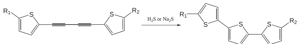
Scheme 1-20: formation of thiophene oligomers from diyne precursors
