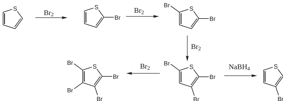
Scheme 1-9: Thiophene bromination
