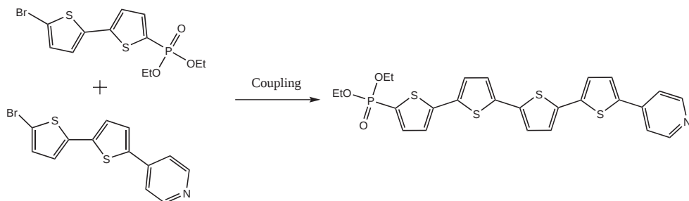
Scheme 6-6: Concept of using bimolecular heterocoupling reaction for the synthesis of a short, asymmetric oligomer
