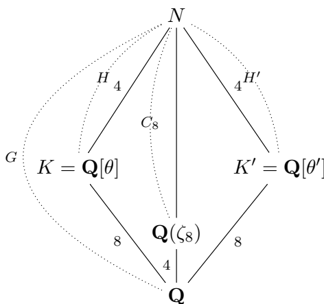
FIGURE 1.1. Perlis' example.
