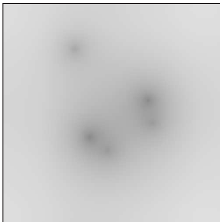
Figure 4.3: Global error map with minimum correction
