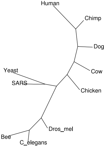
Figure 9.12: Unrooted phylogenetic tree of Table 9.6
