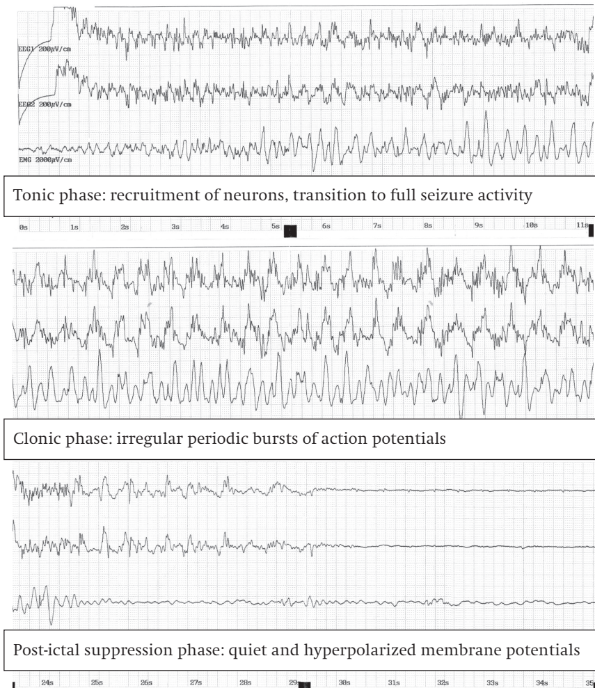
Figure 2 Electroencephalographic registration of seizure activity during electroconvulsive therapy
