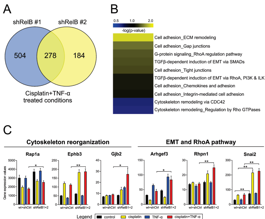
Figure 5. RelB knock-down is associated with up-regulation of RhoA pathway related genes during cisplatin/TNF- \alpha treatment. shCtrl and shRelB cells were exposed to cisplatin (20 \mu M) and/or TNF- \alpha (8 ng/ml) for 8 hours. Following hybridization and RMA normalization, the genes with \geq 1.5 fold-change and FDR \leq 0.1 for shRelB#1 and #2 cell lines compared to wt+ shCtrl cells after cisplatin/TNF- \alpha treatment were further selected. A Venn diagram was made comparing both shRelB cell lines (A). Using the Metacore™ software, pathway analysis was performed on the genes commonly regulated in both shRelB cell lines with cisplatin/TNF- \alpha treatment. The top pathways are represented in a heatmap (B). The gene expression changes of genes involved in cell adhesion, EMT and the RhoA pathway are represented for wt-shCtrl cells combined and both shRelB cell lines combined in cisplatin/TNF- \alpha treated conditions. The statistical significance is indicated only for the conditions where for both shRelB#1 and #2 the fold-change was \geq 1.5 . The data are representative of three independent experiments and expressed as mean \pm S.E.M. * P \leq 0.05 and ** P \leq 0.05 (C).
