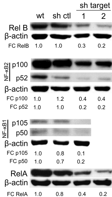
Supplemental Figure 1. Knock-down efficiency of the NF- \kappa B members. The knock-down efficiency of the different NF- \kappa B members was assessed by Western blotting. B-actin was used as a loading control and the quantification indicated is the mean of three independent experiments.
