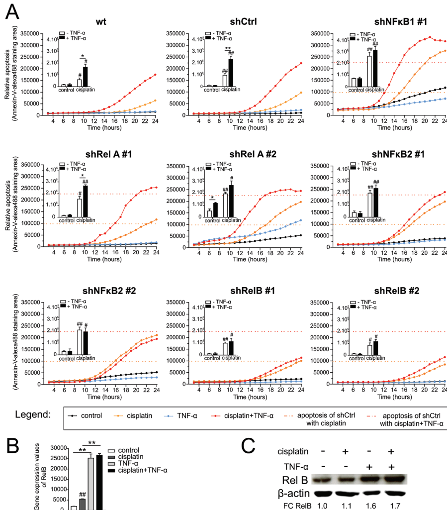
Figure 2. RelB knock-down suppresses cisplatin/TNF- \alpha synergistic apoptosis. IM-PTEC cell lines with knock-down for each NF- \kappa B family member (NF- \kappa B1, NF- \kappa B2, RelA and RelB) were generated using lenti-viral shRNA (see materials and methods). Knock-down cells were exposed to cisplatin (20 \mu M) and/or TNF- \alpha (8 ng/ml). Cell death was followed over time using Annexin V-Alexa488 staining and automated imaging. Both apoptosis overtime and endpoints are represented. The dashed orange and red lines indicate the amount apoptosis observed with shCtrl cells after cisplatin or cisplatin/TNF- \alpha treatment respectively (A). After cisplatin (5 \mu M) and/or TNF- \alpha (8 ng/ml) treatment for 8 hours, the gene expression (B) and protein (C) levels of RelB were assessed. Gene expression values were obtained from previous Affymetrix gene array data (16) (B) and protein levels were assessed by Western blotting (C). B-actin was used as a loading control and the quantification indicated is the mean of three independent experiments (C). The data are representative of three independent experiments and expressed as mean \pm S.E.M. * P \leq 0.05 , ** P \leq 0.01 and # P \leq 0.05 , ## P \leq 0.01 compared to vehicle-treated cells.
