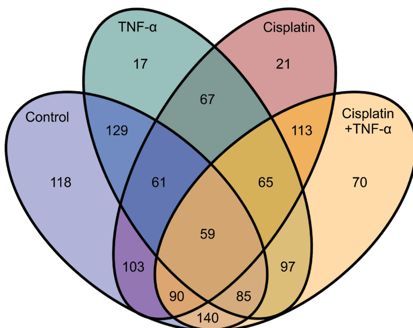
Supplemental Figure 3. Comparison of the differentially expressed genes between treatments. The differentially expressed genes common for both shRelB#1 and #2 cell lines compared to wt+shCtrl cells with fold-change \geq 1.5 or \leq -1.5 and FDR \leq 0.1 are represented for each treatment in a Venn diagram.
