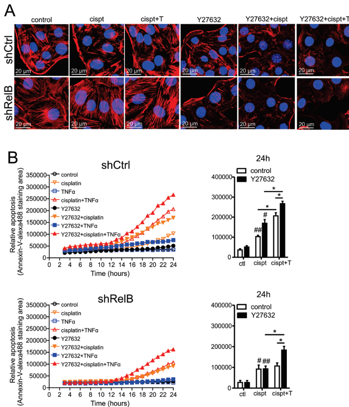
Figure 6. RelB knock-down protects against cisplatin/TNF- \alpha treatment in a Rho kinase dependent manner. shCtrl and shRelB cells were pre-exposed to the ROCK inhibitor Y27632 for 30 minutes prior to cisplatin (20 \mu M) and/or TNF- \alpha (8 ng/ml). After 8 hours of exposures to cisplatin and/or TNF- \alpha in combination with the ROCK inhibitor, actin was visualized by staining of F-actin with rhodaminephalloidin (red). The nuclei were visualized with Hoechst staining (blue). Images of both shCtrl cells and shRelB cells have the same scale as indicated in the images in the bottom right corner (A). Cell death after ROCK inhibition was followed over time using Annexin V-Alexa488 staining and automated imaging (B). ctl=control, cispt=cisplatin and cispt+T=cisplatin+TNF- \alpha . The data are representative of three independent experiments and expressed as mean \pm S.E.M. * P \leq 0.05 and # P \leq 0.05 , ## P \leq 0.01 compared to vehicle-treated cells.
