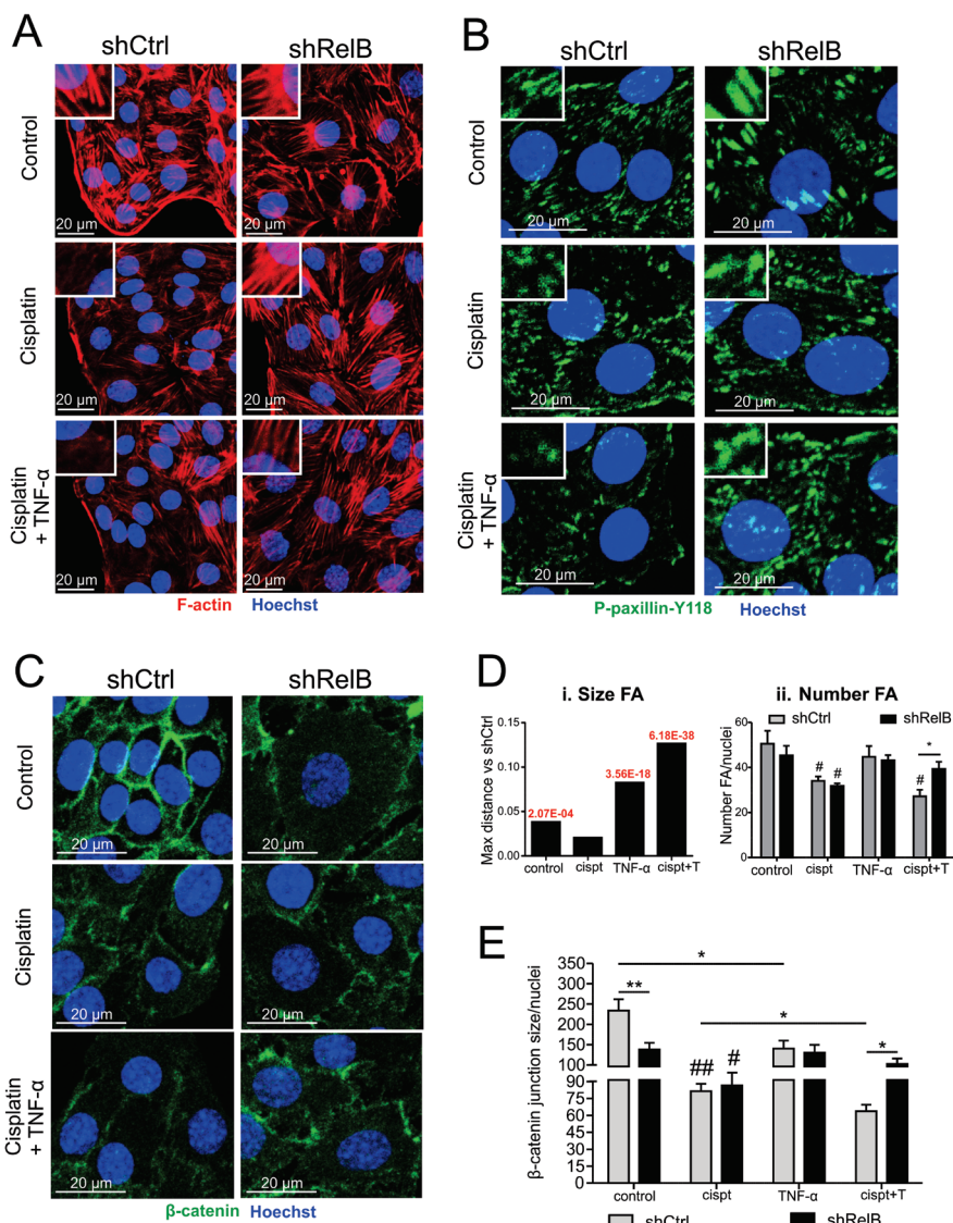
Figure 3. RelB knock-down inhibits cisplatin/TNF- \alpha -induced cell adhesion and actin cytoskeleton changes. shCtrl and shRelB cells were exposed to cisplatin (20 \mu M) and/or TNF- \alpha (8 ng/ml) for 8 hours and immuno-stained to visualize the actin cytoskeleton, focal adhesions and cell-cell adhesions. Cells were imaged using a Nikon TiE2000 confocal microscope. The effect of RelB knock-down on actin cytoskeleton was visualized by staining of F-actin with rhodamine phalloidin (red) (A). The effect of RelB knock-down on focal adhesions was assessed by staining of P-paxillin-Y118 (green) (B). Cell-cell contacts disturbances after treatment were assessed by staining the adherens junction protein \beta -catenin (green) (C). Quantification of P-paxillin (D) and \beta -catenin (E) was performed as described under Fig. 1 and materials and methods. For all images, the nuclei were stained with Hoechst (blue) (A, B and C). Images of shCtrl cells and shRelB cells have the same scale as indicated in the images in the bottom right corner. cispt=cisplatin, cispt+TNF- \alpha and cispt+T=cisplatin+TNF- \alpha . The data are representative of three independent experiments and expressed as mean \pm S.E.M. * P \leq 0.05 and # P \leq 0.05 , ## P \leq 0.01 compared to vehicle-treated cells.
