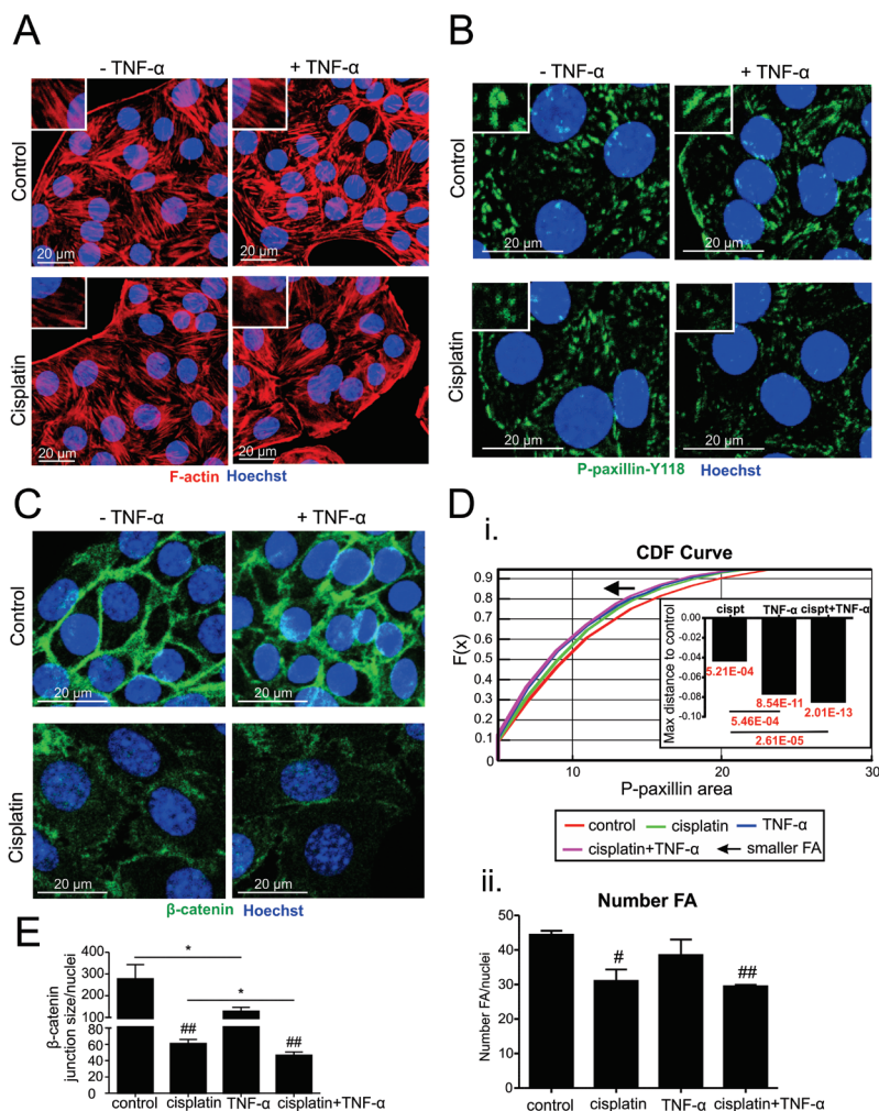
Figure 1. TNF- \alpha aggravates cisplatin-induced disruption of stress fibres, cell-ECM adhesion and cell-cell contacts. IM-PTECs were exposed to cisplatin (20 \mu M) and/or TNF- \alpha (8 ng/ml) for 8 hours and immunostained to visualize the actin cytoskeleton, the focal adhesions and cell-cell adhesions. Cells were imaged using a Nikon TiE2000 confocal microscope. The effect of treatment on the actin cytoskeleton was visualized by staining of F-actin with rhodamine phalloidin (red) (A). The effect of treatment on focal adhesions (FA) was assessed by staining of P-paxillin-Y118 (green) (B). Quantification of P-paxillin was performed. The CDF curve indicates the direction of the changes in focal adhesion size with the different treatments. A KS test was performed relative to control treatment and indicates the differences observed in P-paxillin size between cisplatin and/or TNF- \alpha treated cells and vehicle-treated cells. The p-values obtained are indicated in red. The number of focal adhesion was also assessed by quantifying P-paxillin fluorescence per cell (D). Cell-cell contacts disturbances after treatment were assessed by staining the adherens junction protein \beta -catenin (green) (C), which was quantified by assessing the average area occupied by \beta -catenin per cell (E). For all images, the nuclei were stained with Hoechst (blue) (A, B and C). Images of shCtrl cells and shRelB cells have the same scale as indicated in the images in the bottom right corner. The data are representative of three independent experiments and expressed as mean \pm S.E.M. * P \leq 0.05 and # P \leq 0.05 , ## P \leq 0.01 compared to vehicle-treated cells.
