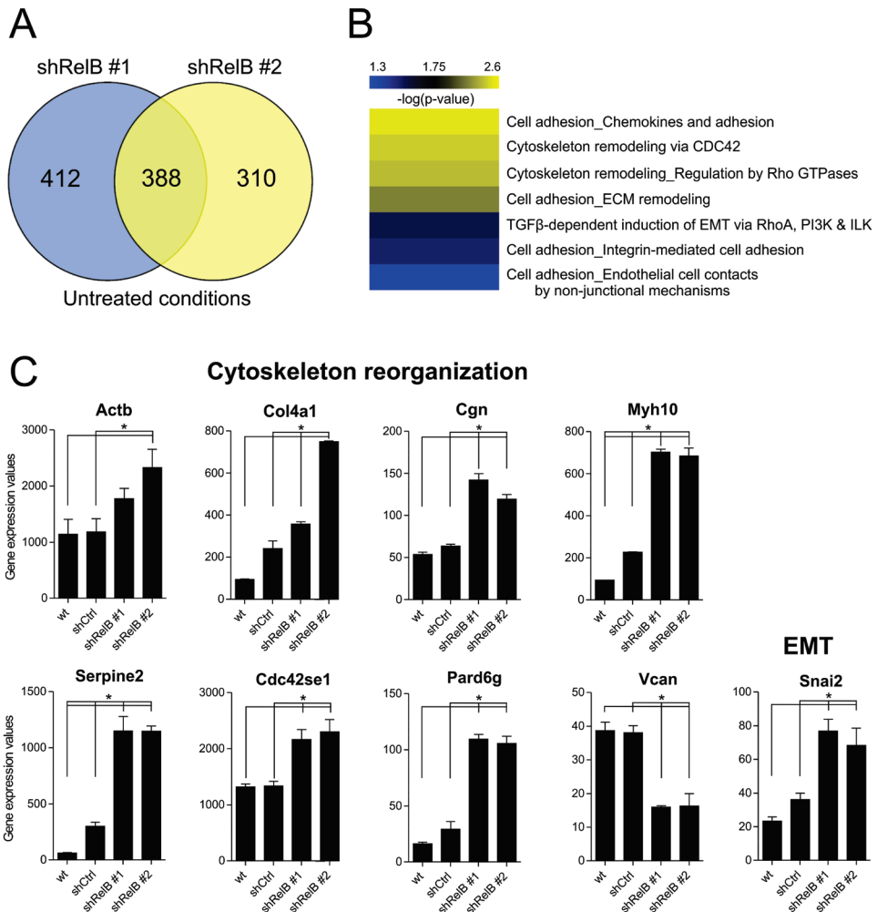
Figure 4. RelB knock-down leads to EMT-like driven cytoskeletal rearrangements in vehicle-treated cells. shCtrl and shRelB cells were exposed to cisplatin (20 \mu M) and/or TNF- \alpha (8 ng/ml) for 8 hours. Following hybridization and RMA normalization, the genes with \geq 1.5 fold-change and FDR \leq 0.1 for shRelB #1 and #2 cell lines compared to wt+ shCtrl cells in control conditions were further selected. A Venn diagram was made comparing both shRelB cell lines in control conditions (A). Using the Metacore™ software, pathway analysis was performed on the genes commonly regulated in both shRelB cell lines in control conditions. The top pathways are represented in a heatmap (B). The gene expression changes of genes involved in cytoskeleton organization and EMT are represented for wt and shCtrl as well as both shRelB cell lines in control conditions. The data are representative of three independent experiments and expressed as mean \pm S.E.M. * P \leq 0.05 (C).
