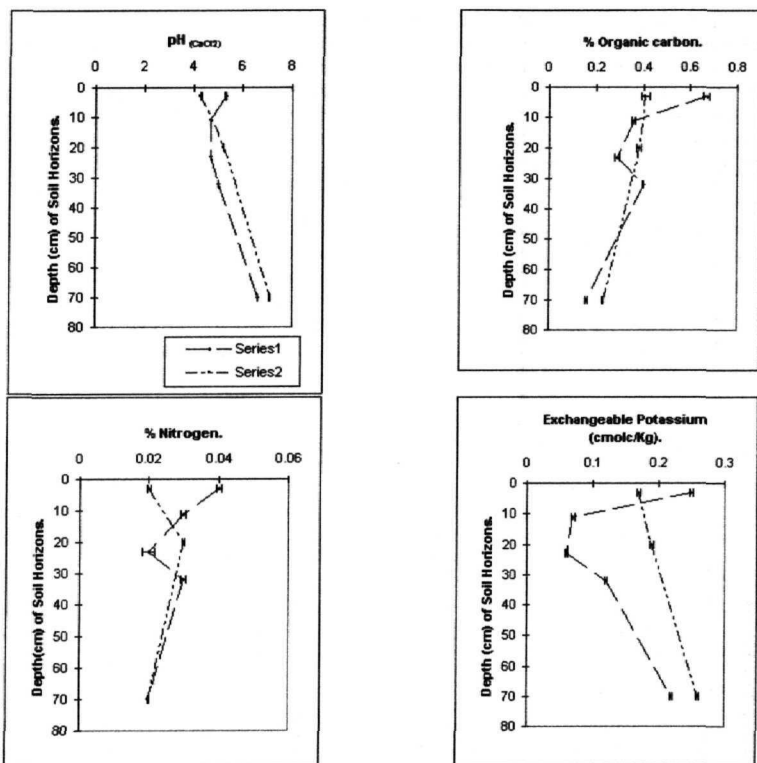
Figure 4.2: Impacts of land use histories on the mean values ( n=4 ) of some chemical properties of the horizons in the Eutric Planosol.
