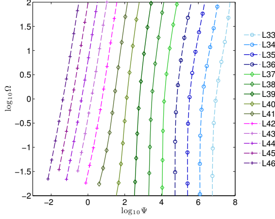
Figure 5.1 – An example of how our models fill the parameter space of \Psi and \Omega . In the Figure, each plot symbol shows the values of \Psi and \Omega computed for a particular calculation in our model grid at t = 0 , n_{\text{H, in}} = 10 \text{ cm}^{-3} , with radiation pressure on. Colors indicate lines of constant L , running from 10^{33} - 10^{46} \text{ erg s}^{-1} as indicated in the legend. The sequence of points along a given model corresponds to varying R_{\text{in}} from 10^{-2} \tilde{r}_{\text{ch}} - 10^2 \tilde{r}_{\text{ch}} , with \Omega increasing with R_{\text{in}} . Note that \Psi is a function of density as well as ionizing source luminosity. Radiation pressure can be significant in a high density region with relatively lower ionizing luminosity. Note that our full H II region model grids are incorporated into the dynamical models in Paper II.
