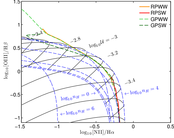
Figure 5.2 – Models in the BPT diagram. Full lines show one-zone models with constant \mathcal{U} , while dashed lines show one-zone models of constant n_{\text{H}} ; both are calculated for an ionizing spectrum corresponding to a zero-age stellar population and Solar metallicity. We also show models RPWW, RPSW, GPWW, and GPSW (as indicated by the legend) with n_{\text{H,in}} = 10 \text{ cm}^{-3} , calculated with the same ionizing spectrum and metallicity.
