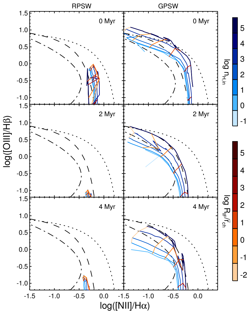
Figure 6.4 – Same as Figure 6.3, but for the strong-wind Models GPSW and RPSW.
