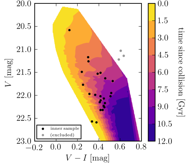
Figure 5.3: Contours of collision time t_{\text{col}} located in the observational colour-magnitude space. The points represent the innermost 27 BSSs, where the three grey points are the stars excluded from our analysis as they sit beyond the TAMS.
