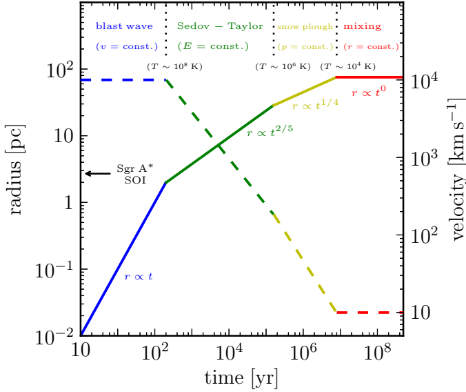
Figure 1.1: The stages of evolution of a supernova remnant for an energy of 10^{51} erg, an ejecta mass of 1 M_{\odot} for a typical ISM ambient density of n_{\text{H}} \sim 1 \text{ cm}^{-3} . Temperatures, T , are given at each of the timescales of the transitions. The solid line shows the evolution of the radius, while the dashed line shows the evolution of the velocity. (More realistically, the evolution is ‘intermediate-asymptotic’, transitioning between these limiting functions.) The scale of the sphere of influence of the Milky Way supermassive black hole, Sgr A*, is indicated with an arrow. [After Padmanabhan, 2001, Figure 4.6]
