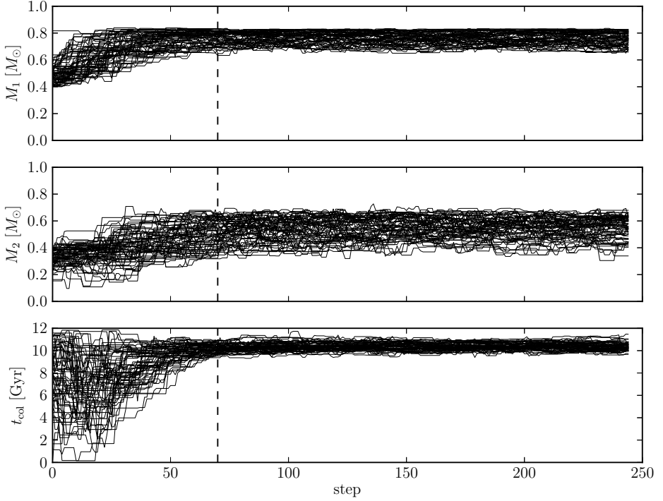
Figure 5.5: Positions of walkers used for the MCMC run for inner BSS 1. The parameters from top to bottom are: the mass of the more massive star, the mass of the less massive star, and the collision time. The black dashed line shows the cut for the chain burn-in; positions prior to this are not used for the final statistics.
