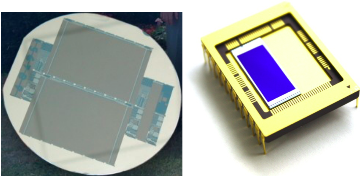
Figure 6.12 — Left: e2v Gaia silicon wafer with photoactive regions (dark grey) showing two CCD91-72s in the centre and small test structures on either side. The photoactive strip on the right side is two CCD221s abutted. Right: Gaia test structure CCD221 packaged for use. (Images courtesy of e2v technologies.)
