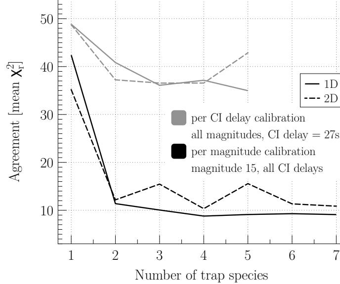
Figure 5.4 — Comparison between the mean agreement obtained after performing a per magnitude (black) and a per CI delay (grey) calibrations of the CDM parameters using different number of trap species and performing the CDM simulation in 1D (continuous line) or 2D (dashed line). In the per magnitude calibration case (black), the test data used to perform the calibration contains 10 damaged over-sampled profiles with G = 15 and different CI delays ranging from 30 ms to 120 s. In the per CI delay calibration case (grey), the test data used to perform the calibration contains 5 damaged over-sampled profiles for a CI delay of 27 s and for G = 13.63, 15.29, 16.95, 18.65, 20.25 .
