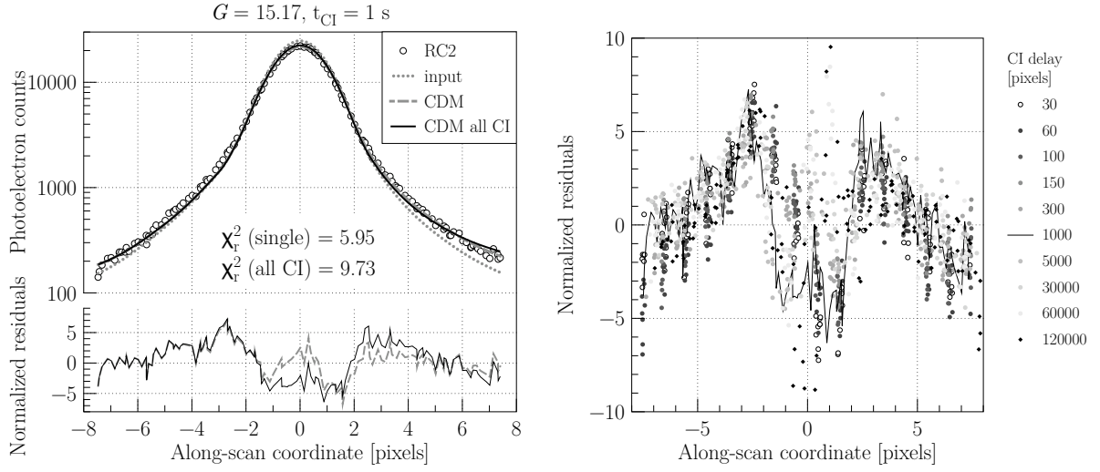
Figure 5.3 — Left: Comparison between the RC2 test data (black circles) and two CDM predictions for the same signal level ( G \sim 15 ) and CI delay ( \sim 1 \text{ s} ). The dashed grey line is a CDM prediction for a parameter set (Table 5.2 column 4) obtained after an individual fit to the depicted RC2 profile, whereas the continuous black line is the CDM prediction for a parameter set (Table 5.2 column 5) obtained after a simultaneous fit to 10 damaged profiles with different CI delays including the one depicted. The dotted grey curve corresponds to the CDM input signal in both cases.
