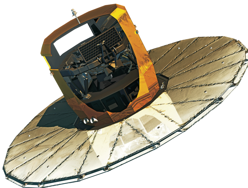
Figure 1.4 — General view of the Gaia spacecraft with the deployed sun shield. The cut-out in the thermal tent allows one to see: the payload and its two primary mirrors mounted on the mechanically and thermally stable torus (top), the service module (bottom). The satellite height is \sim 3 m and, once deployed, the sun shield diameter reaches 10 m. Illustration courtesy of EADS Astrium
