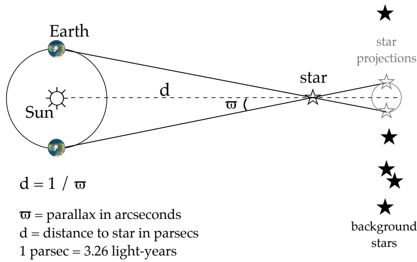
Figure 1.1 — Schematic representation of the stellar parallax and its measurement using the diameter of the Earth's as the baseline. The parallactic motion is depicted by the small grey circle. It is the apparent motion of the star of interest with respect to background (more distant) stars. The parallactic motion is periodic and mirrors the Earth's orbit around the Sun as seen from the star of interest.
