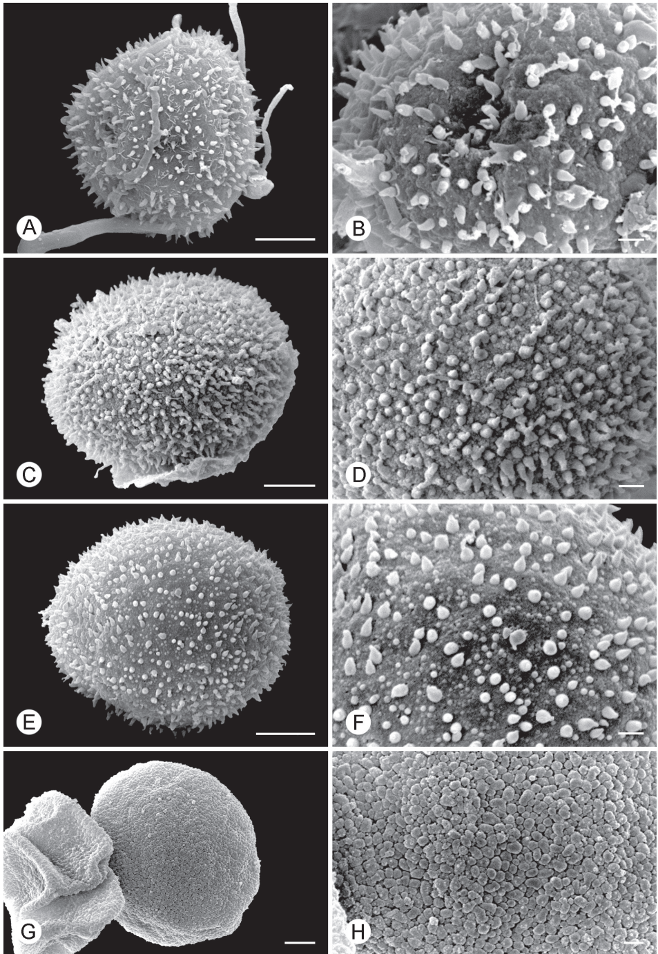
FIGURE 5. Pollen of Neo-uvaria and Enicosanthum , SEM. A, B. Neo-uvaria foetida : (A) Pollen grain, showing
