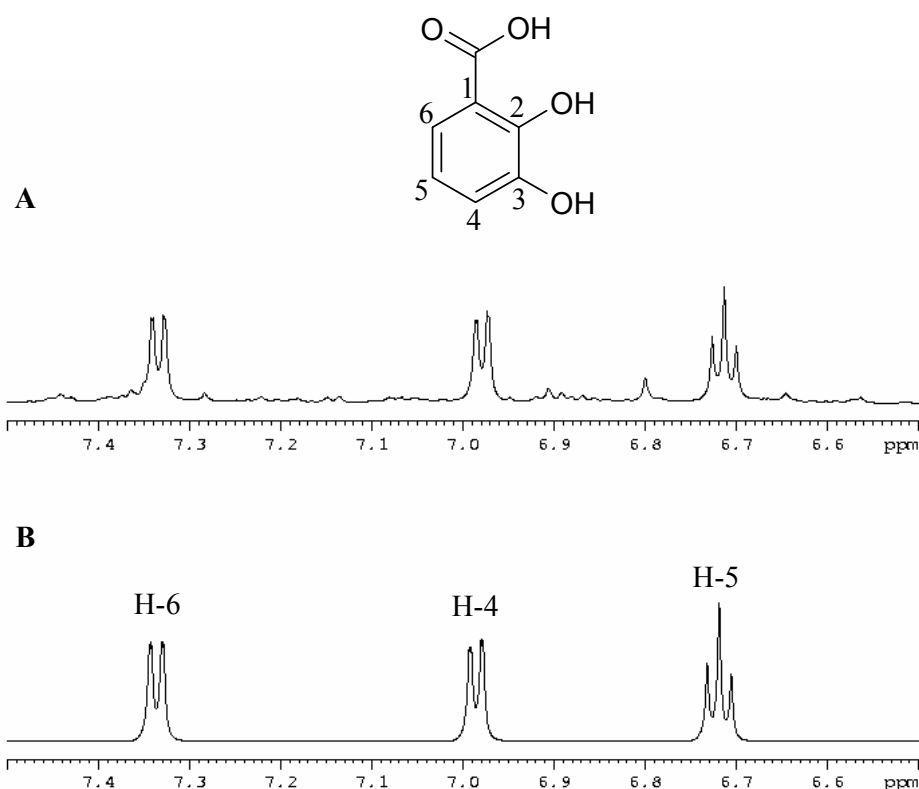
Figure 6.7. ^1\text{H} -NMR spectra ( \text{CH}_3\text{OH}-d_4 ) of medium containing enriched 2,3-DHBA of batch 1 of Catharanthus roseus suspension cultures elicited by Pythium (A) and of 2,3-DHBA standard (B, 10 mg/mL).
