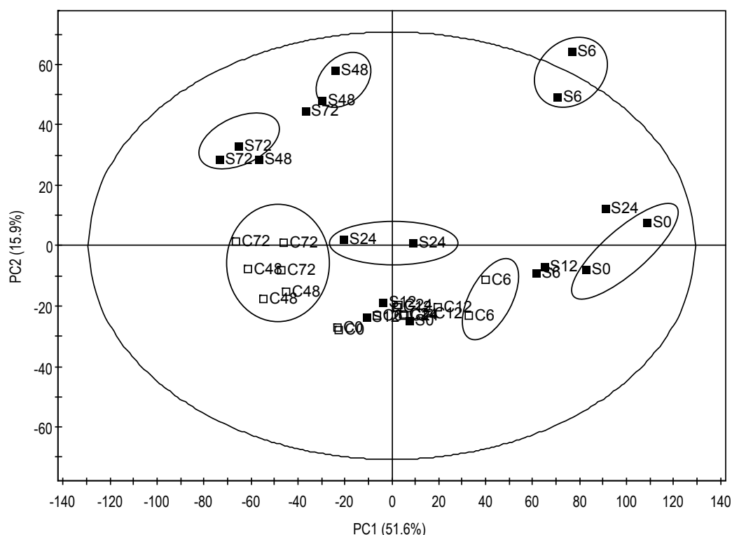
Figure 7.1. The score plot of PCA of ^1\text{H} -NMR data of Catharanthus roseus cells extracted with \text{CH}_3\text{OH}-d_4\text{-KH}_2\text{PO}_4 in \text{H}_2\text{O}-d_2 pH 6.0 (1 : 1). C: control cells, S: SA-treated cells, the number after the symbol shows the observation time (hour) after treatment.
