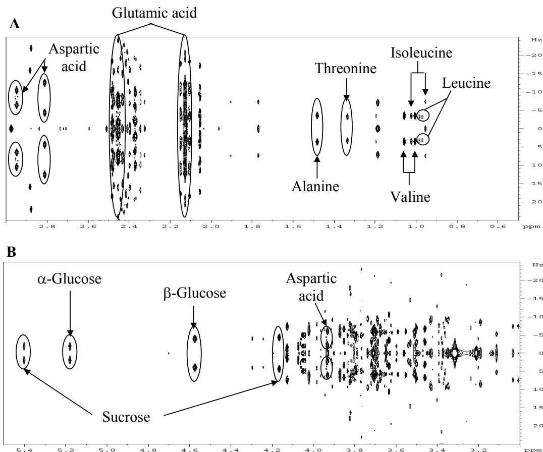
Figure 7.3. Some metabolites signals in the aliphatic region (A) and sugars region (B) of J-resolved ^1\text{H} -NMR spectrum ( \text{CH}_3\text{OH}-d_4\text{-KH}_2\text{PO}_4 in \text{H}_2\text{O}-d_2 pH 6.0, 1 : 1) of the extract of Catharanthus roseus cells 12 h after elicitation with sodium-SA.
