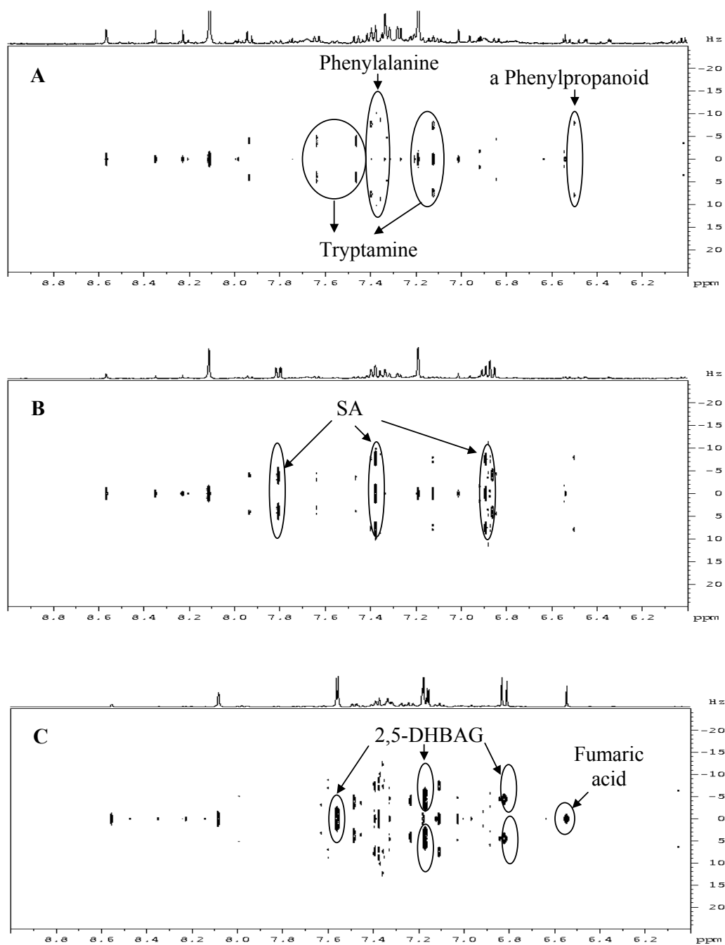
Figure 7.4. The signals of some compounds in the aromatic region of J-resolved ^1\text{H} -NMR spectra of Catharanthus roseus cells extracted with \text{CH}_3\text{OH}-d_4\text{-KH}_2\text{PO}_4 in \text{H}_2\text{O}-d_2 pH 6.0 (1 : 1). A: 6 h-control cells, B: 6 h-elicited cells, C: 48 h-elicited cells. SA= salicylic acid, 2,5-DHBAG= 2,5-dihydroxybenzoic acid glucoside.
