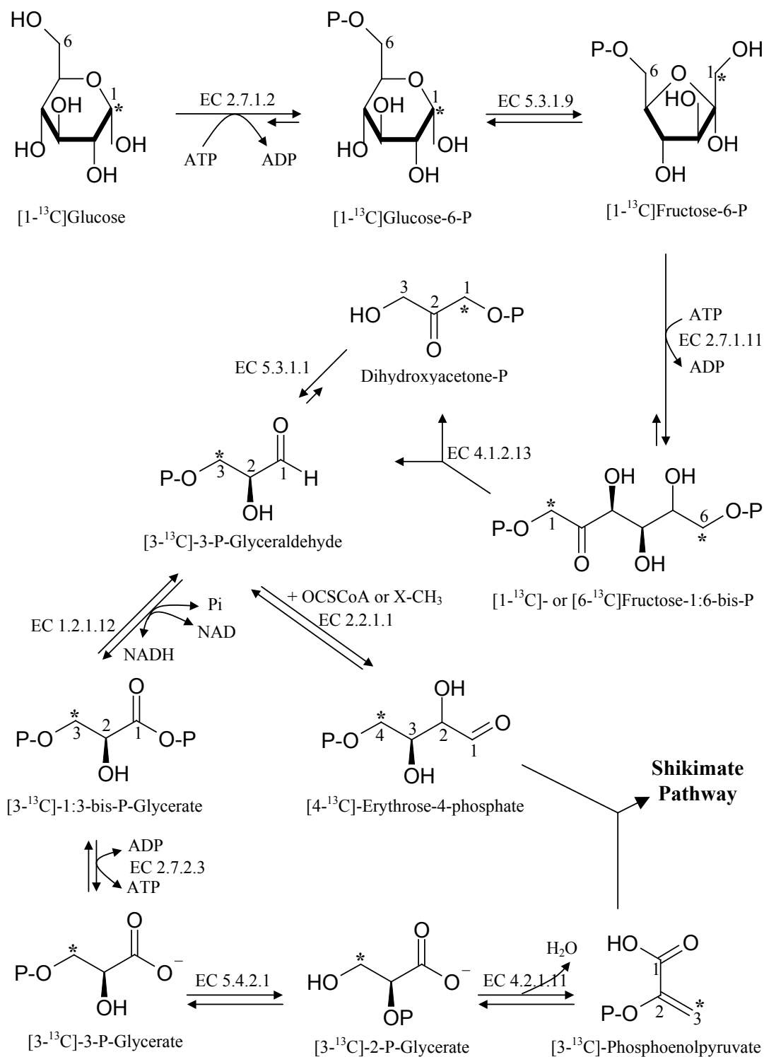
Figure 6.1. Glycolysis/ Embden-Meyerhof-Parnas
